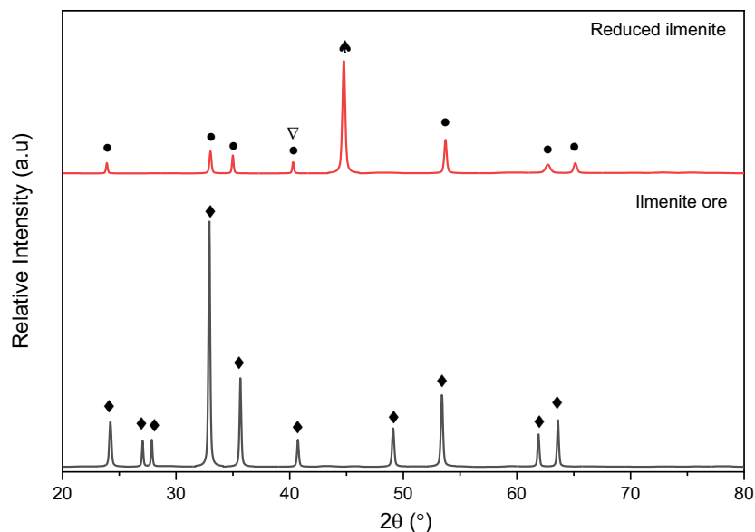
Fig. 2. The XRD diffractogram pattern of the unreduced ilmenite (raw ilmenite ore) and the reduced ilmenite. (♦ FeTiO 3 ; ● Ti 2 O 3 ; ▲ Fe; ▽ TiC)
