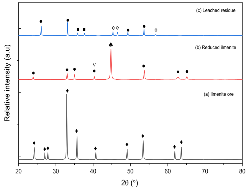
Fig. 7. XRD diffractogram patterns of the (a) ilmenite ore, (b) reduced ilmenite and (c) leached residue. (♦ FeTiO 3 ; • Ti 2 O 3 ; ▲ Fe; ▽ TiC; ■ Fe 2 O 3 ; ◇ Ti 3 O 5 )
