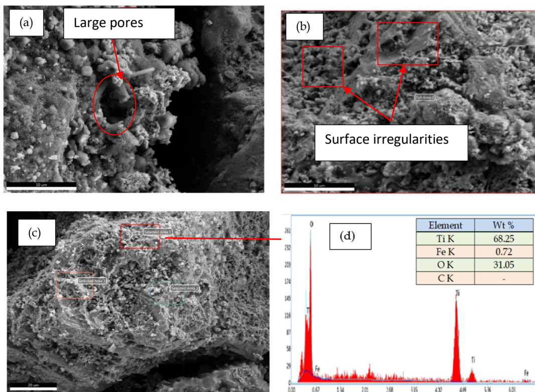
Fig. 8. SEM photomicrograph of the leached residue (90°C, 7 hours in 0.5M NH 4 Cl) (a) surface morphology of the porous structure; (b) surface irregularity; (c) and (d) EDX spot analysis
