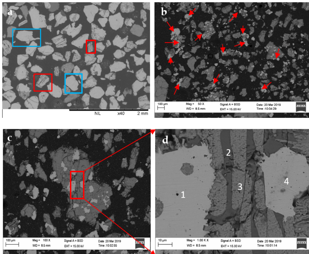
Fig. 1. Backscattered electron photomicrograph of the (a) raw ilmenite ore, (b) reduced ilmenite at carbon to oxygen molar ratio 1:1.4, (c) reduced ilmenite grains and (d) reduced ilmenite
