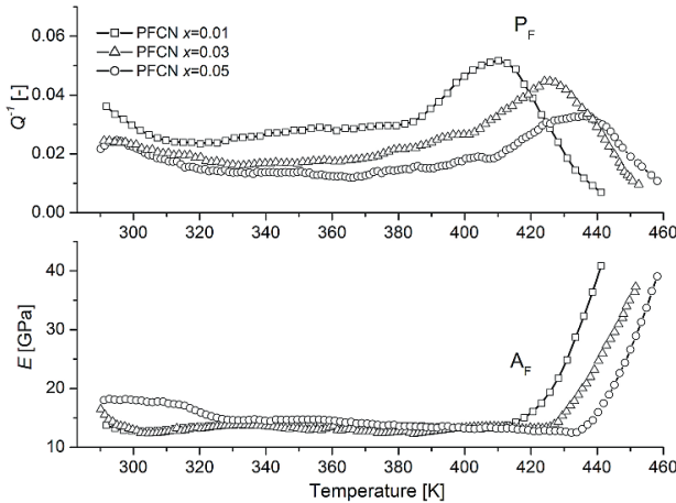
Fig.2. Temperature relationships of the Q^{-1}(T) internal friction and the E(T) dynamic Young's modulus of the admixed PFCN ceramics for x = 0.01, 0.03 and 0.05 ( f = 753 Hz).
