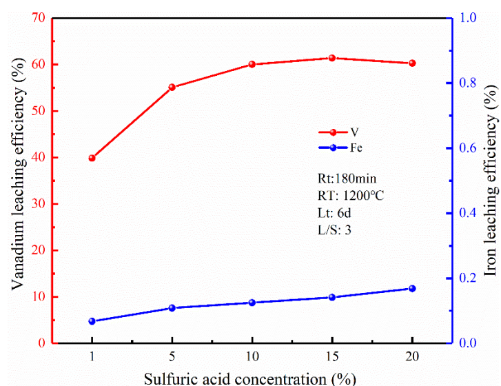
Fig. 10. Effect of sulfuric acid concentration on the leaching efficiency of V and Fe
