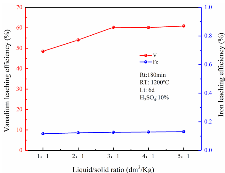
Fig. 9. Effect of liquid/solid ratio on the leaching efficiency of V and Fe
