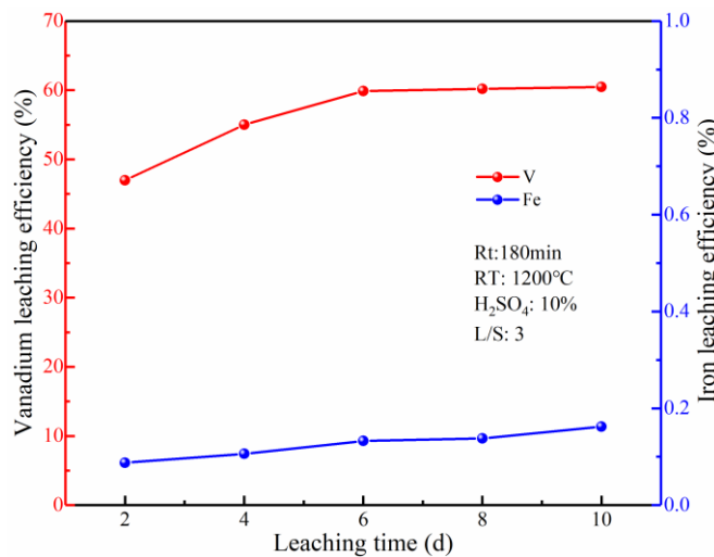
Fig. 8. Effect of leaching time on the leaching efficiency of V and Fe
