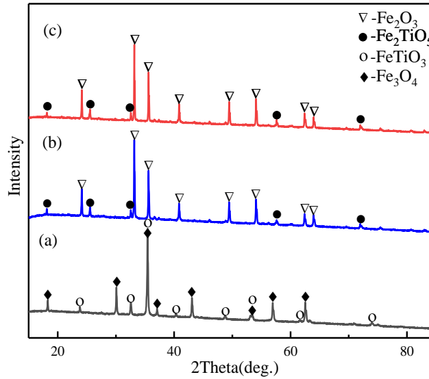
Fig. 12. XRD pattern of pellet samples: (a) concentrate, (b) roasted pellets, and (c) leached pellets
