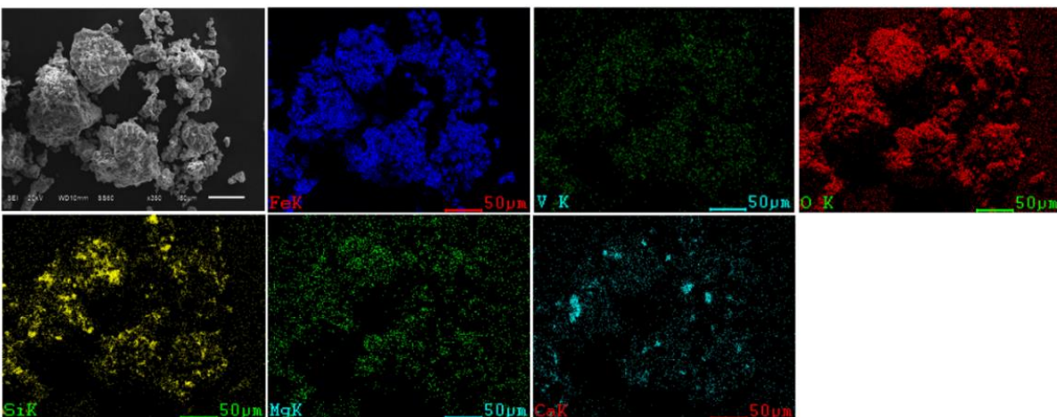
(b) Leaching pellets
