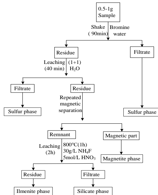
Fig. 2. Phase analysis process of vanadium in vanadium-titanium magnetite
