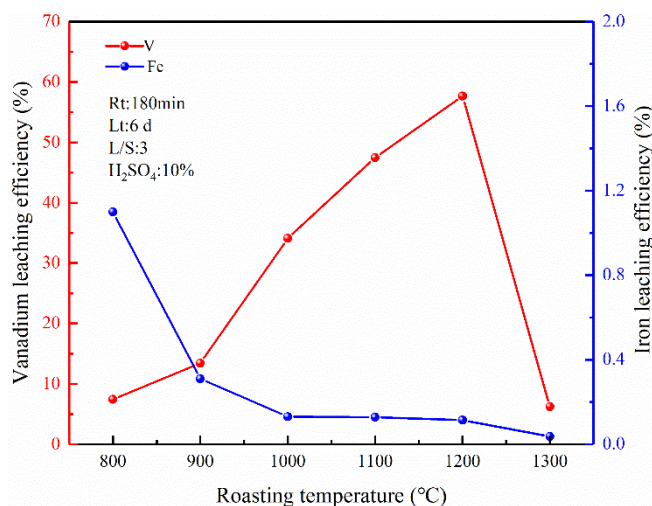
Fig. 6. Effect of roasting temperature on the leaching efficiency of V and Fe
