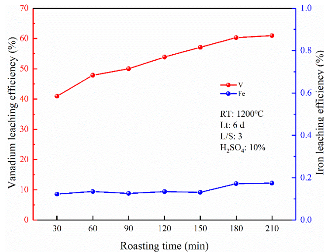
Fig. 7. Effect of roasting time on the leaching efficiency of V and Fe
