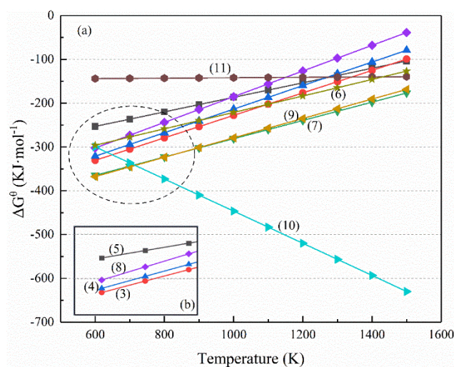
Fig. 5. \Delta G^\theta -T diagrams for possible chemical reactions (Eqs. 3-11)
