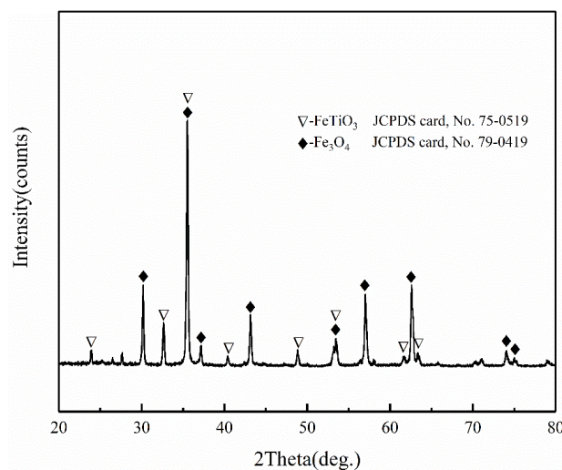
Fig. 3. XRD pattern of vanadium-titanium magnetite concentrate
