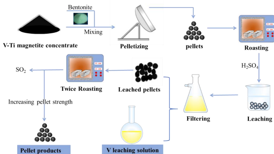
Fig. 1. Process chart of the non-salt roasting-pellet acid leaching
