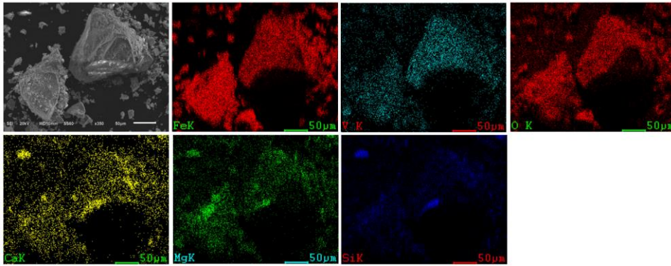
Fig. 4. SEM images with EDS element mapping of the concentrate
