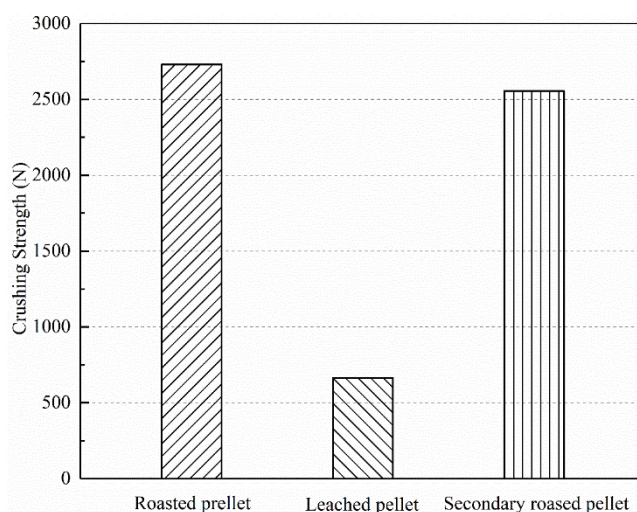
Fig. 11. Crushing strength of roasted pellets, leached pellets and secondary pellets
