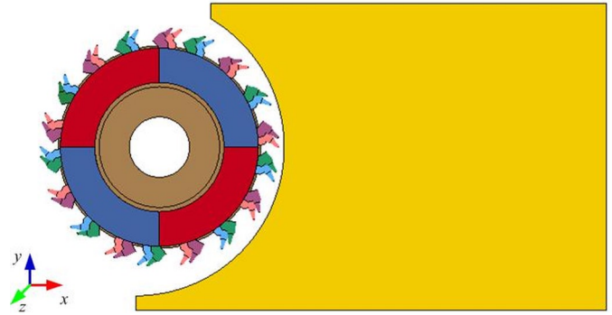
Fig. 6. Finite element model of drum cutting coal
