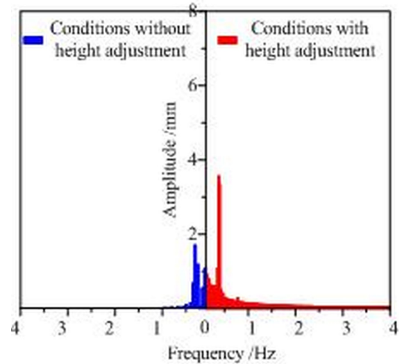
Fig. 11. Amplitude-frequency characteristics of drum vibration
