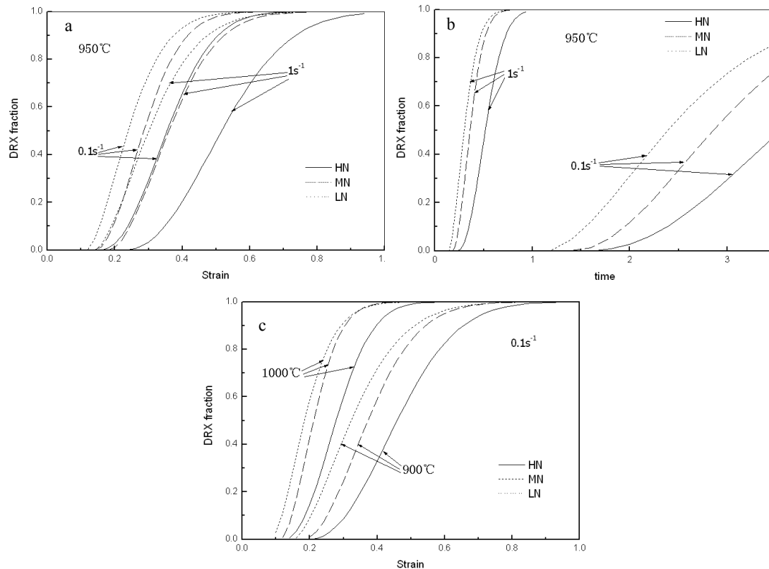
Fig. 5. Relation between DRX volume fractions and (a) strain at 950°C (b) deformation time at 950°C (c) strain at 0.1\text{ s}^{-1}
