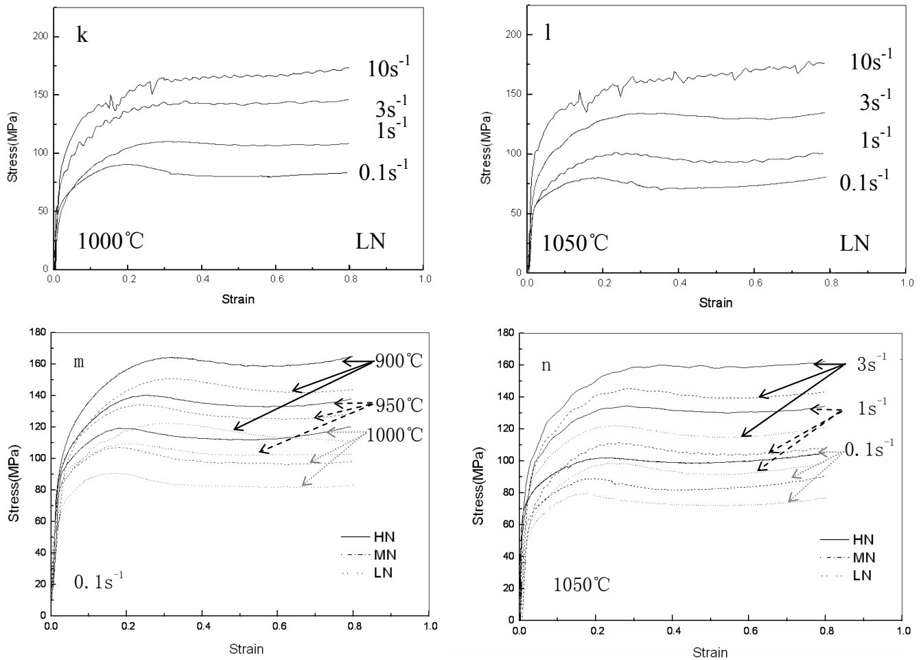
Fig. 1. True stress-strain curves of the experimental steels deformed under various deformation conditions (a), (b), (c) and (d) Curves for high nitrogen steel (HN); (e), (f), (g) and (h) Curves for medium nitrogen steel (MN); (i), (j), (k) and (l) Curves for low nitrogen steel (LN); (m) and (n) Comparison of the curves for the experimental steels
