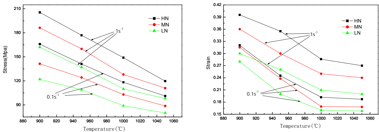
Fig. 2. Relation between temperature and peak stress (a) or peak strain (b)
