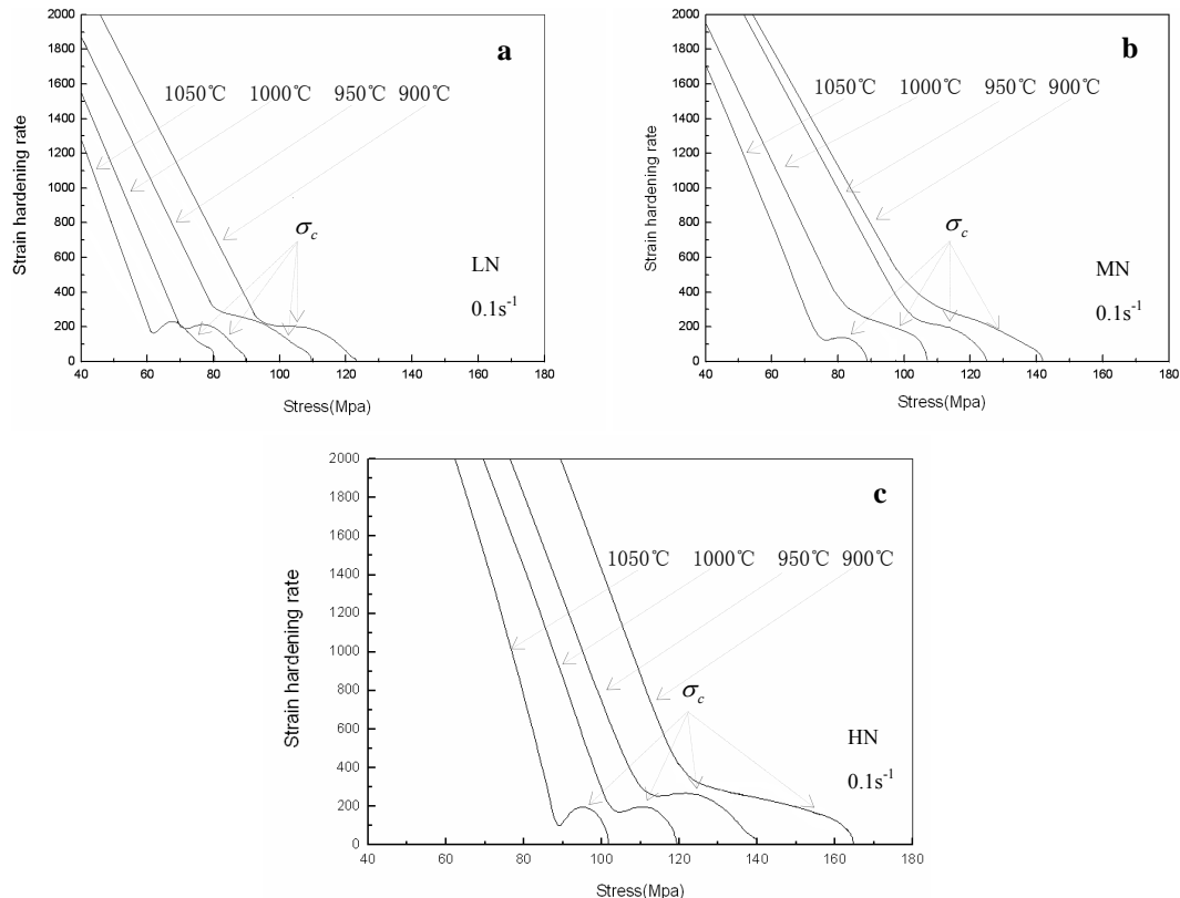
Fig. 3. Strain hardening versus stress curves of the tested steel (a) low nitrogen steel (b) medium nitrogen steel (c) high nitrogen steel
