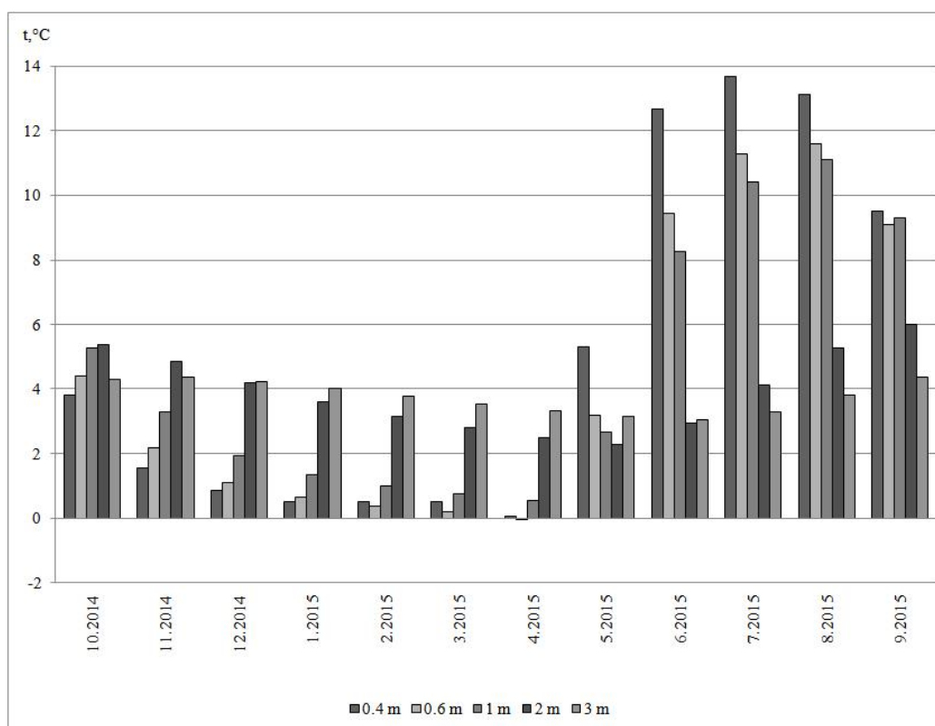
Fig.2. Soil Temperature for Thermowell 6 (Natural Area) for 2014-2015
