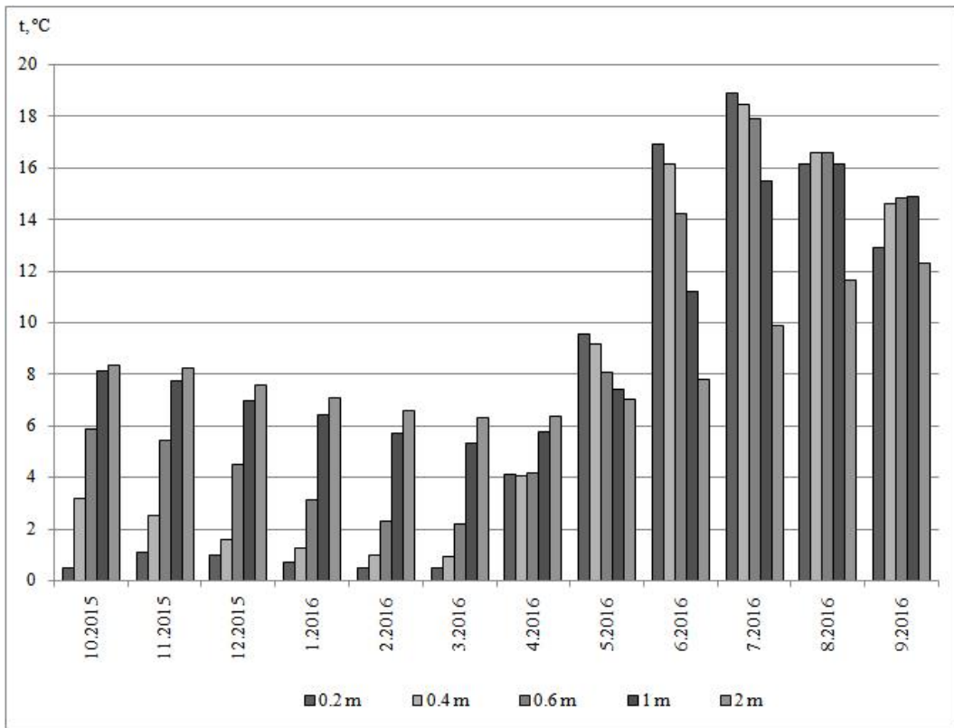
Fig.5. Mean Temperatures for Thermowells 5a (Natural Area) for 2015-2016
