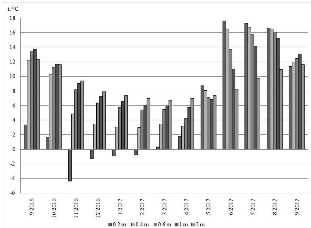
Fig.7. Summary Graph of Mean Temperatures for Thermowell 5a (Technogenic Area) for 2016-2017
