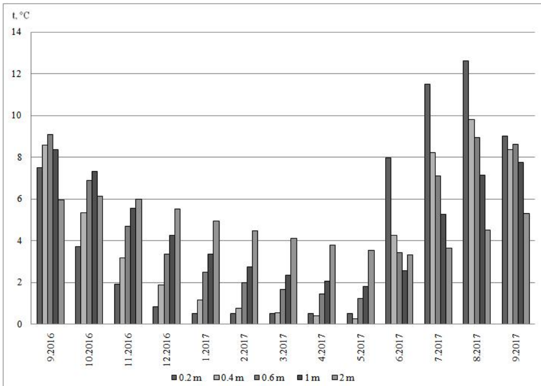
Fig.6. Mean Temperatures for Thermowells 5 (Natural Area) for 2016-2017
