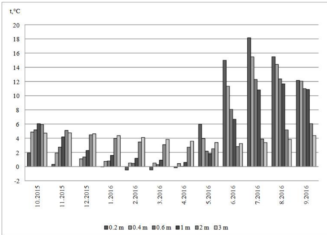
Fig.3. Soil Temperature for Thermowell 6 (Natural Area) for 2015-2016
