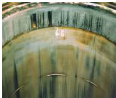
Fig. 4. Image of the damaged surface of cylinder liner due to an excessive friction wear resulting from the seizing of piston in the cylinder [30]
