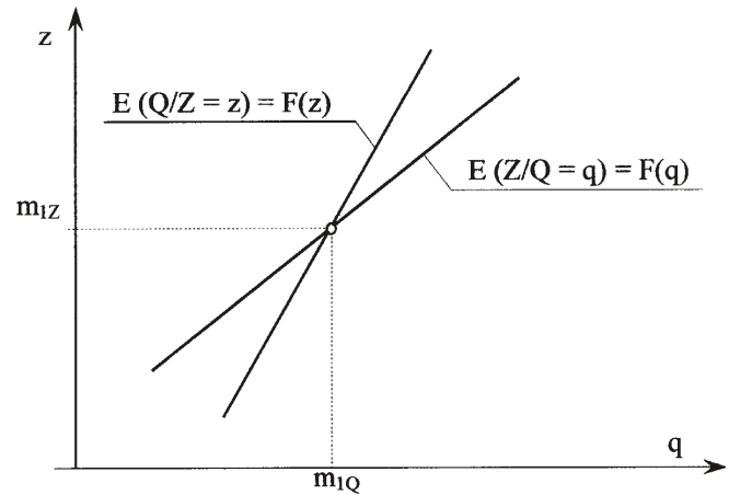
Fig. 10. Graphical illustration of the course of regression straight lines: m_1 - 1^{\text{st}} order zero moment (expected value), m_{1Z} = E(Z) , m_{1Q} = E(Q) , respectively; E(Q/Z=z) - expected value of the variable Q dependent on the value z of the variable Z , E(Z/Q=q) - expected value of the variable Z dependent on the value q of the variable Q , z - realization of the variable Z (wear), q - realization of the variable Q (load).
