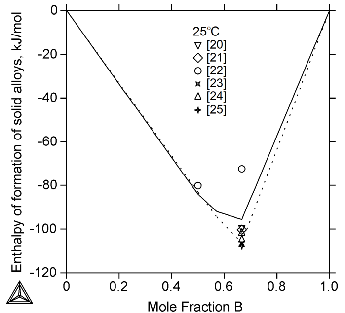
Fig. 5. Calculated enthalpy of formation of solid B-Ti alloys at 25°C, together with experimental data points [20-25]. Solid line refers to the current calculations and dotted line refers to those of Bätzner [11]. The reference states used are pure hcp Ti and pure beta-rhombo B
