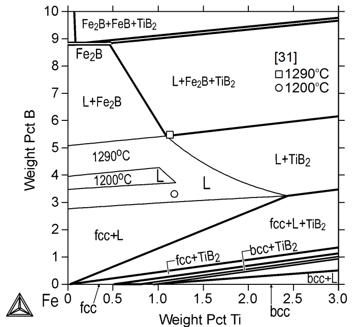
Fig. 9. Calculated isotherm of 1290°C in the Fe-B-Ti system, together with an experimental data point for the liquid phase [31]. Shown also is the liquid phase at 1200°C, with an additional experimental data point from [31]
