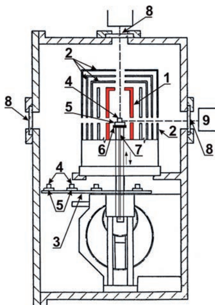
Fig. 3. A schematic presentation of the wettability testing equipment by the sessile drop method combined with CH procedure: 1 – Mo heater, 2 – Mo screens, 3 – rotating loading table, 4 – alloy, 5 – substrate, 6 – experimental table with up and down movement, 7 – thermocouple, 8 – observation window, 9 – high-speed CCD camera [8]
