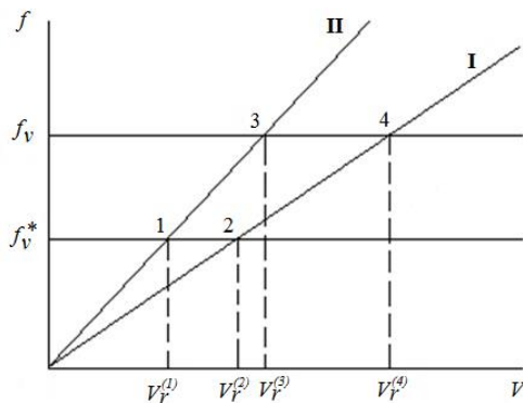
Fig. 1. Scheme for determining resonant velocities
