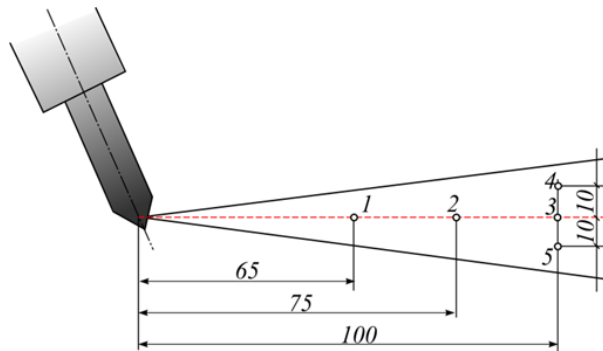
Fig. 7. Distribution of measurement points in the atomised fuel stream
