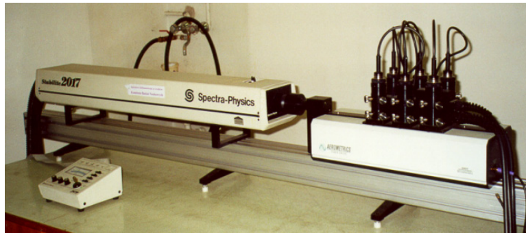
Fig. 1. View of 3-Beam Spectra Physics Laser and Bragg Cell
