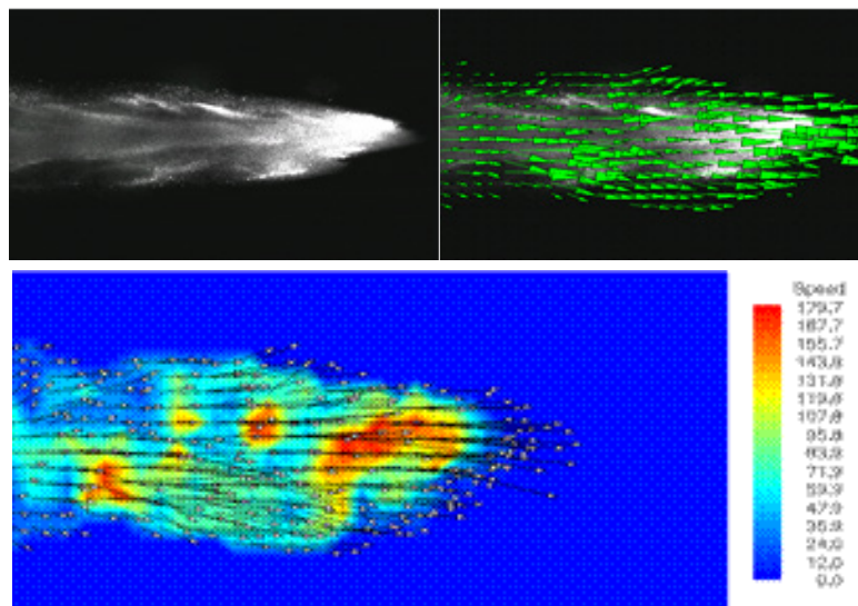
Fig. 6. PIV Flow Pattern with Velocity Vectors for No. 1 Fuel at 100 MPa Pressure
