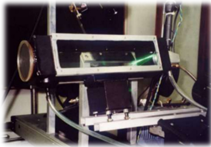
Fig. 8. View of the test chamber Source: own development
