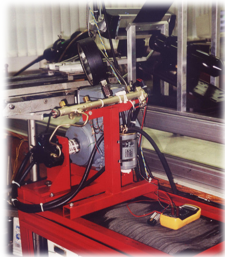
Fig. 9. Common rail injection system Source: own development
