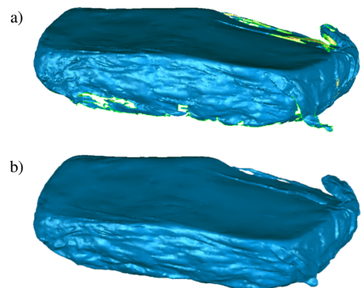
Fig. 7. Comparison before and after model repair. Irregular rubber block model: a) without filling and b) with filling
