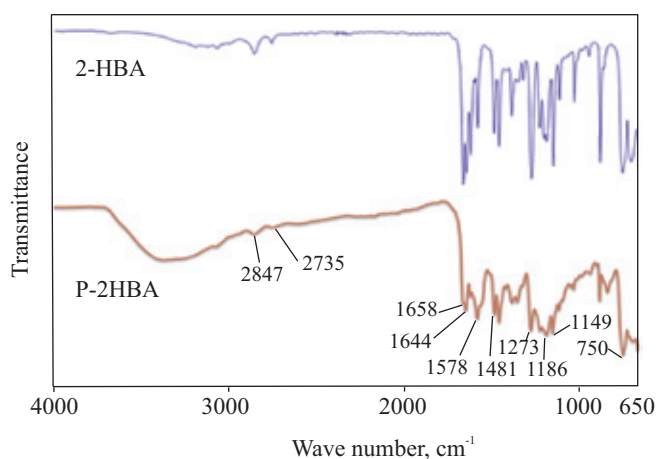
Fig. 1. FT-IR spectra of 2-HBA and P-2HBA
