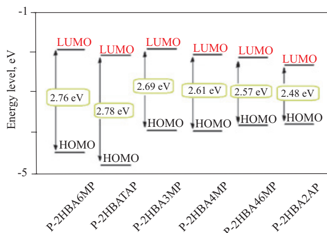
Fig. 5. HOMO-LUMO energy levels and electrochemical band gaps of the polymers
