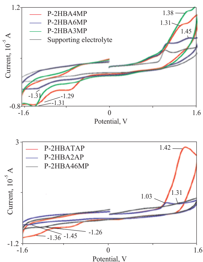
Fig. 4. Cyclic voltammograms of the polymers
