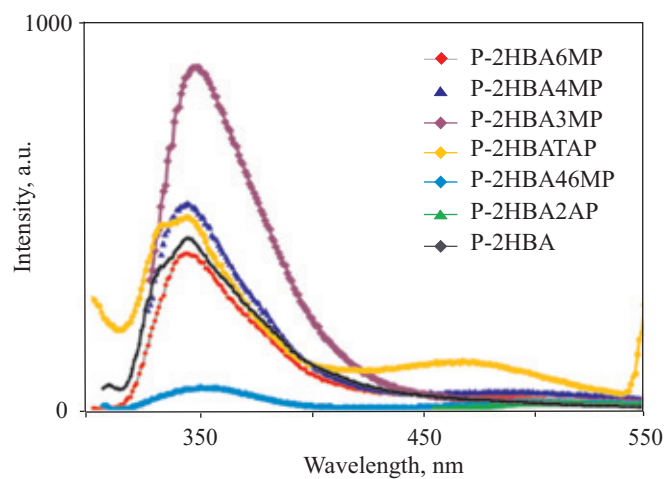
Fig. 8. Emission spectra of solutions in DMF (slit width: \lambda_{Ex} = 5 \text{ nm} , \lambda_{Em} = 5 \text{ nm} ; concentration of the compounds: 0.001 \text{ g/dm}^3 )
