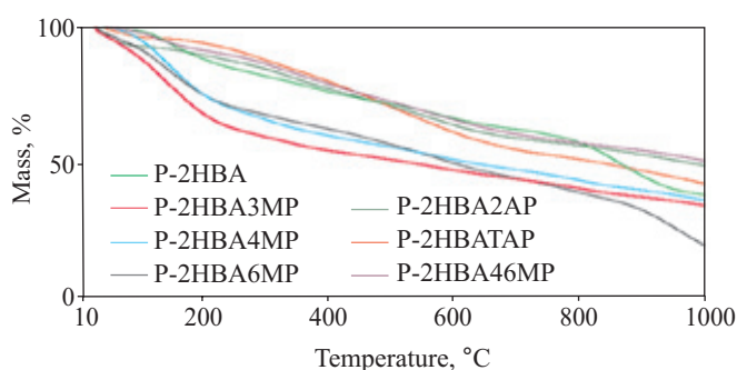
Fig. 3. TGA curves of the polymers
