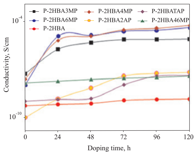
Fig. 7. Electrical conductivity changes of the I_2 -doped at 25 °C
