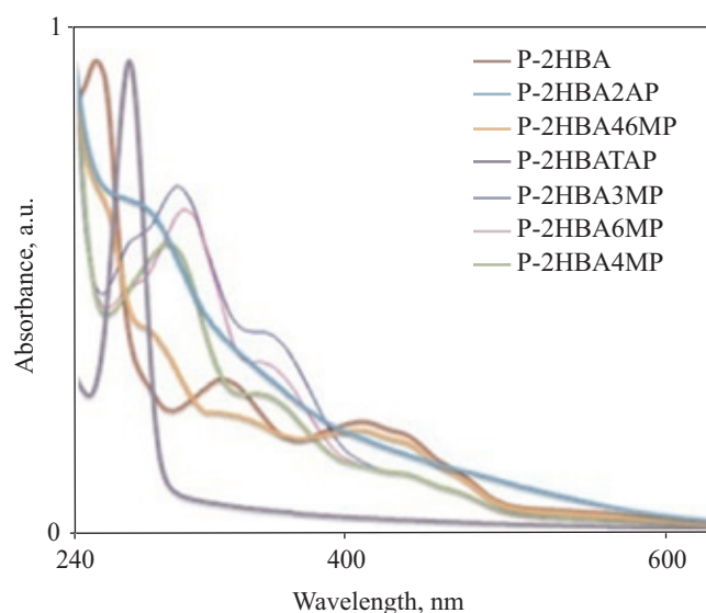
Fig. 6. UV-Vis spectra of the polymers
