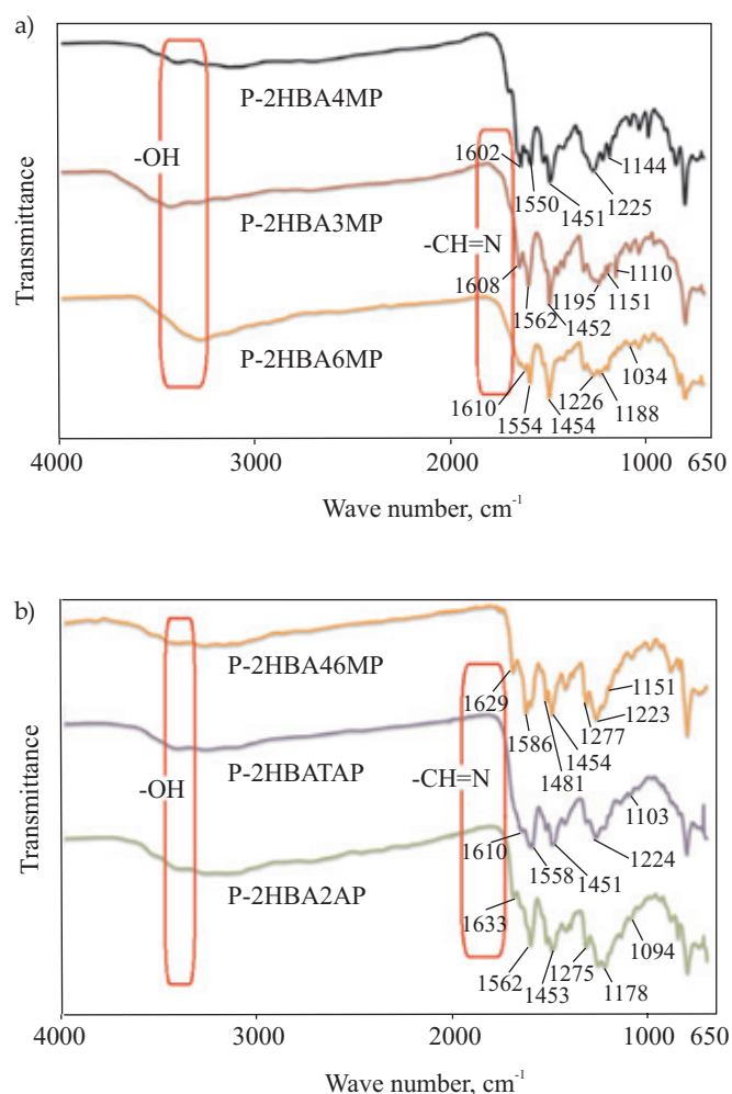
Fig. 2. FT-IR spectra of poly Schiff bases containing: a) pyridine, b) pyrimidine
