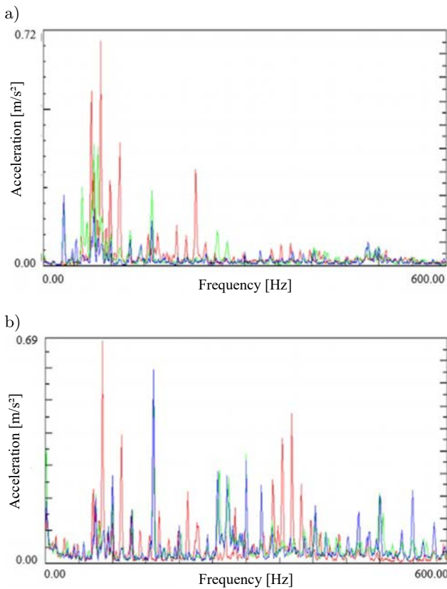
Fig. 13. Acceleration FFT of AC pipe (a) and compressor (b) in the HVAC model; red – AC off, green – AC on without TDVA, and blue – AC on with TDVA (idle).
