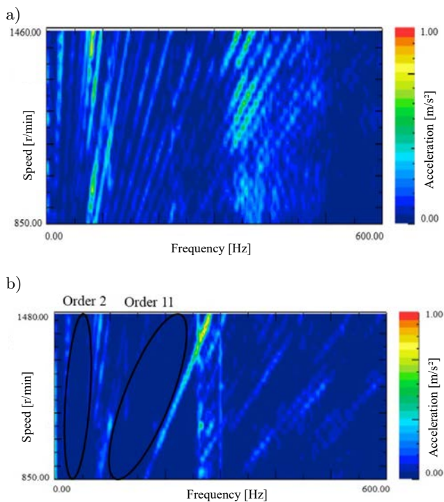
Fig. 10. 3D colour map acceleration of compressor when AC is off (a) and AC is on (b) in the HVAC model (operating).
