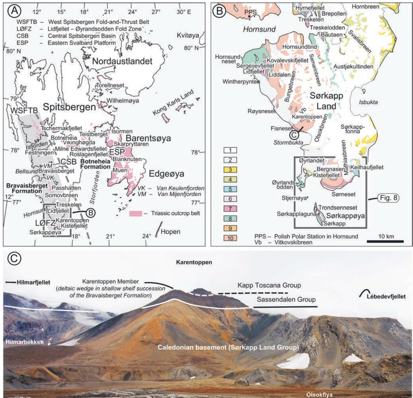
Fig. 1. The Bravaisberget Formation (Middle Triassic–Carnian) in Spitsbergen, Svalbard. A. Map of Svalbard showing outcrops of the Triassic succession in the West Spitsbergen Fold-and-Thrust Belt (WSFTB), including the Lidfjellet–Øyrandsodden Fold Zone (LØFZ), and in the Eastern Svalbard Platform (ESP), including central Spitsbergen. These two developments are separated by the Palaeogene Central Spitsbergen (foreland) Basin (CSB). The suggested boundary between the areas of occurrence of the Botneheia and Bravaisberget formations (the youngest formations in the Sassendalen Group) is marked by a dashed line. The Triassic outcrop belt after Dallmann et al. (2002), modified. B. Geological map of Sørkapp Land. The area enlarged in Fig. 8 is marked by a rectangle. Geology after Winsnes et al. (1993), Dallmann et al. (1993b, 2002), Krajewski and Stempień-Sałek (2003), and unpublished materials of the present authors, simplified. 1 – ice and snow cover; 2 – Quaternary sediments; 3 – Van Mijenfjorden Group (Palaeogene); 4 – Helvetiafjellet and Carolinefjellet formations (Early Cretaceous); 5 – Janusfjellet Subgroup (Late Jurassic–Early Cretaceous); 6 – Kapp Toscana Group (Late Triassic–Middle Jurassic); 7 – Sassendalen Group (Early Triassic–Carnian); 8 – Billefjorden, Gipsdalen and Tempelfjorden groups (Carboniferous–Permian); 9 – Adriabukta Formation (Devonian); 10 – Caledonian basement. C. Central part of the Sørkapp-Hornsund High shows the Triassic succession of the Sassendalen and Kapp Toscana groups resting directly on the Caledonian substratum; here at Karentoppen between Vitkovskibreen and Olsokbreen. The Bravaisberget Formation shows the presence of deltaic deposits (Karentoppen Member) in the shallow-marine succession, which reflect event of supply of clastic material from a land area located southwest of the present coast of southern Spitsbergen. This is the stratotype for the Karentoppen Member (Mørk et al. , 1999). Photograph taken from Fisneset.
