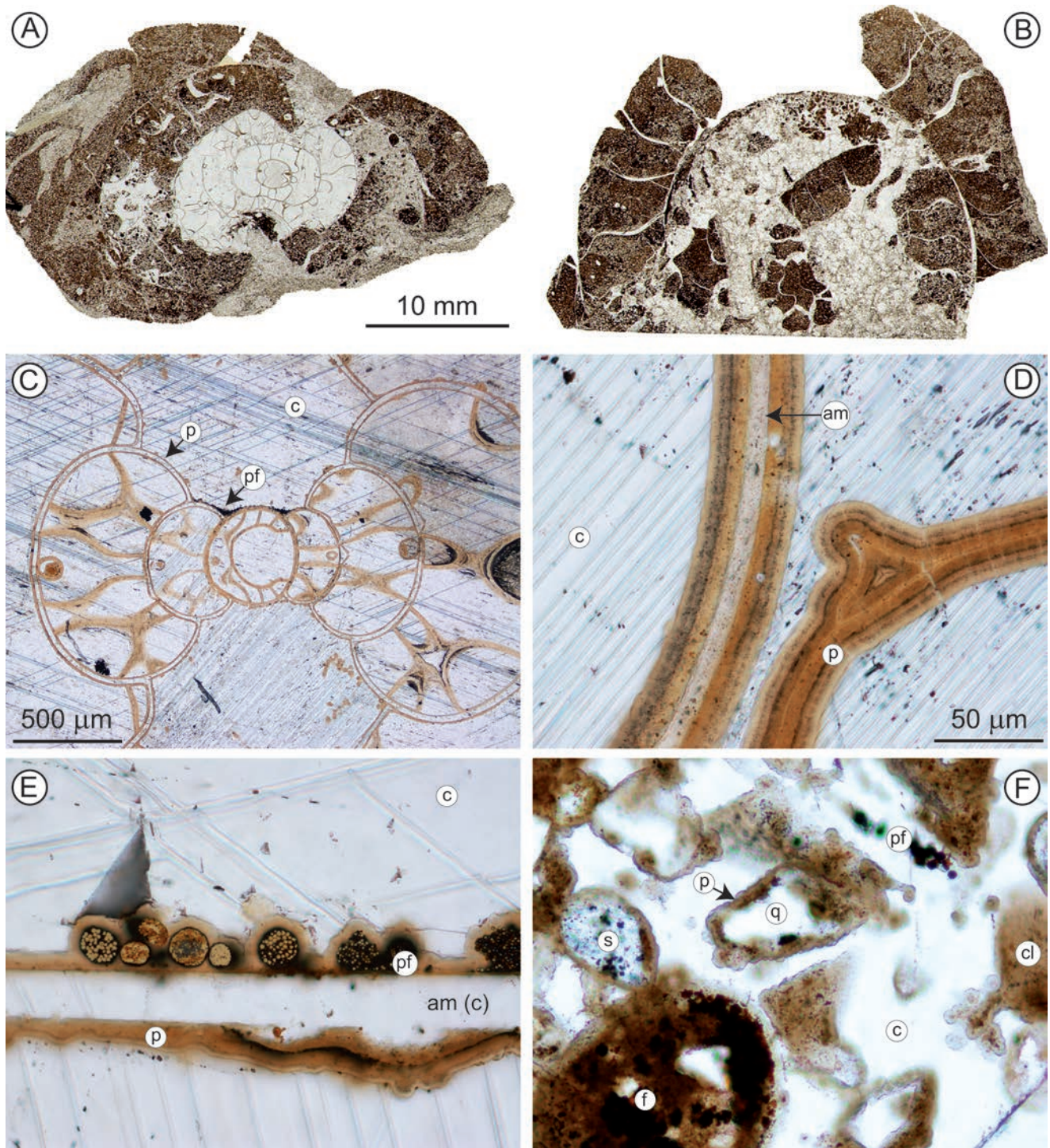
Fig. 12. Phosphatic ammonoids in the Somovbreen Member of the southernmost Sørkapp Land. A. Pristine phosphatic ammonoid in KL section. Note the compactional injection structure of sandy sediment developed in the lower part of internal rings before calcite cementation of the voids. B. Reworked phosphatic ammonoid in KL section. Mechanical fragmentation of the phosphatic infilling occurred before calcite cementation of the voids. C. Carbonate fluorapatite fringe cement ( p ) in internal rings of phosphatic ammonoid contributes to perfect imprint of the original phragmocone anatomy. Note small geopetal structures made of polyframboidal pyrite ( pf ). The remaining pore space and mouldic pores after dissolution of the skeleton are filled by blocky calcite cement ( c ). D. Multilayered apatite fringe cement with seams of pyritic microcrystals ( p ) coating ammonoid septum ( am ). The septum was dissolved during early diagenesis and infilled by a sequence of phosphate and calcite cement. Void space in the phragmocone was infilled by later blocky calcite ( c ). E. Apatite fringe cement ( p ) with pyrite framboids ( pf ) developed on ammonoid septum ( am ). The mouldic pore after dissolution of the septum and the internal void were infilled with later blocky calcite ( c ). F. Clastic sediment filling ammonoid phragmocone shows apatite fringe cement ( p ) on detrital quartz grains ( q ) and moulds of siliceous sponge spicules ( s ), and apatite impregnations of faecal pellets ( f ). Cluster-like apatite cement ( cl ) and polyframboidal pyrite ( pf ) are seen in inter-particle pore space. The remaining voids were filled by calcitic sparite ( c ). (A, B) – thin-section photographs; (C–F) – combined transmitted- and reflected-light photomicrographs, parallel nicols. Scales in (A) and (D) are for (A, B) and (D–F), respectively.
