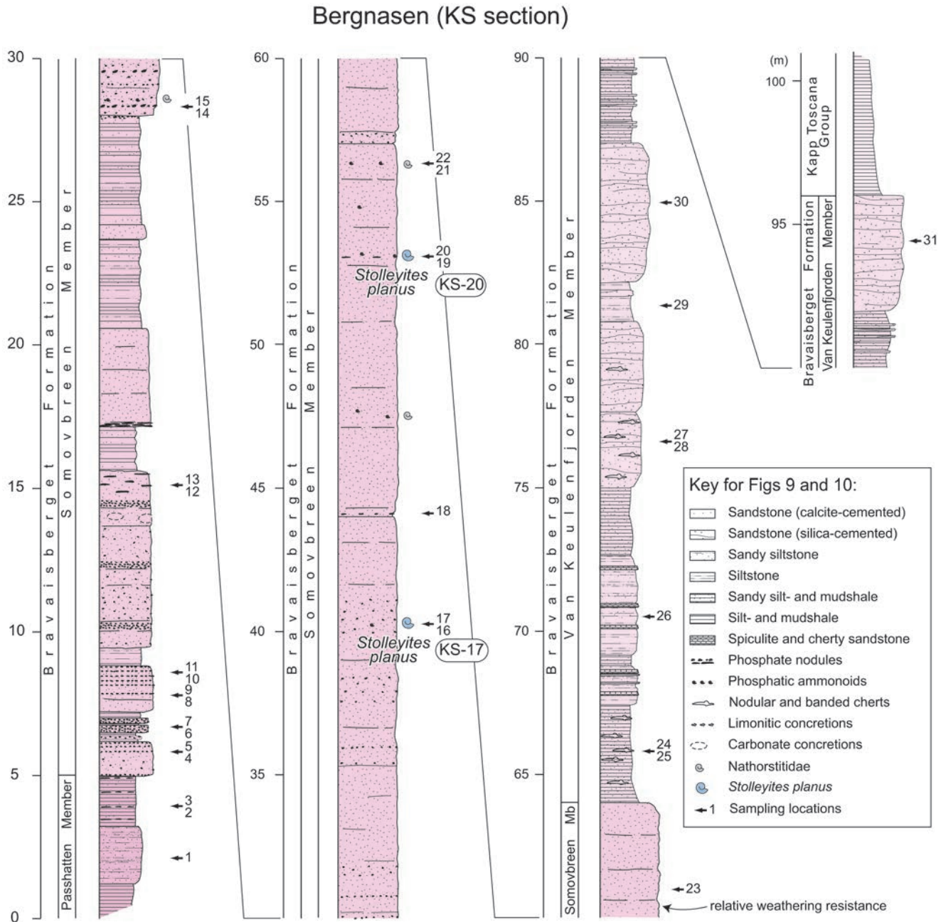
Fig. 9. Bergnasen (KS) section of the Bravaisberget Formation. Findings of Stolleyites planus are indicated. For further explanation, see text.
