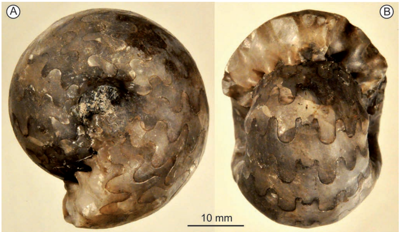
Fig. 13. Stolleyites planus (Frebold). A, B. Sample KL-1C.1 from KL section at Keilhaufjellet (see Fig. 10 for sample location). Calcite-filled middle ontogenetic stage. The suture lines are accentuated by thin apatite fringe cement.
