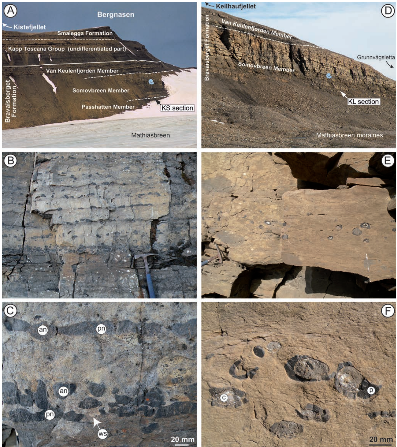
Fig. 11. Lithostratigraphy and facies of the Bravaisberget Formation in the vicinity of Mathiasbreen. A. Eastern slope of Bergnasen showing lithostratigraphic subdivision of the Triassic succession and the direction of KS section of the Bravaisberget Formation. Location of findings of Stolleyites planus is indicated. B. Lower part of the Somovbreen Member at Bergnasen showing succession of fine-grained sandstone with recurrent rows of phosphate nodules. Hammer is 40 cm long. C. Rows of pristine ( pn ) and allochthonous ( an ) phosphate nodules separated by winnowed surface ( ws ) in the lower part of the Somovbreen Member at Bergnasen. D. Rocky cliff at foot of the western slope of Keilhaufjellet showing direction of KL section of the Bravaisberget Formation. Location of findings of Stolleyites planus is indicated. E. Phosphatic horizon in the upper part of the Somovbreen Member at Keilhaufjellet consists of phosphatic ammonoids preserved at various stages of mechanical reworking. Section perpendicular to bedding. Hammer is 40 cm long. F. Ammonoids in phosphatic horizon shown in (E). The external parts of the fossil moulds are cemented by phosphate ( p ), and the internal rings are filled with later blocky calcite ( c ).
