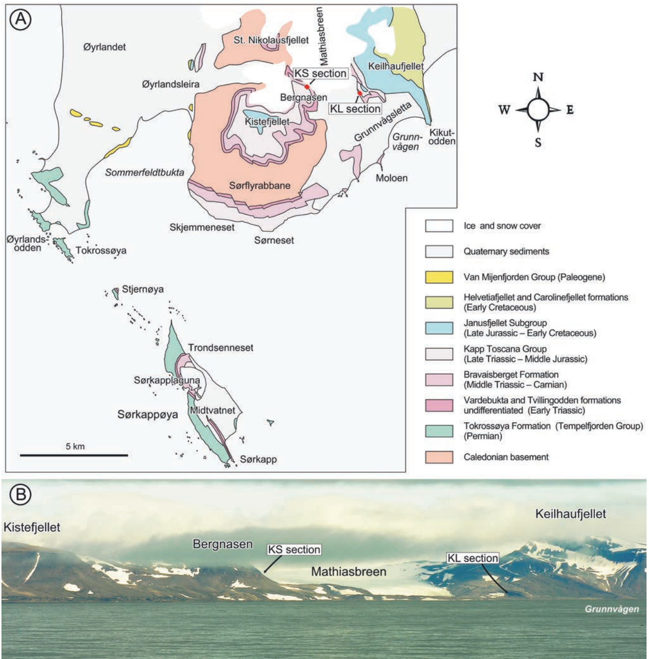
Fig. 8. The Bravaisberget Formation (Middle Triassic–Carnian) in southernmost Spitsbergen. A. Geological map of the southernmost part of Spitsbergen showing location of the Bergnåsen (KS) and Keilhaufjellet (KL) sections of the Bravaisberget Formation. Geology after Winsnes et al. (1993), Dallmann et al. (1993b, 2002), and unpublished materials of the present authors, simplified. B. Panoramic photograph of the southern coast of Sørkapp Land, showing location of KS and KL sections on the western and eastern sides of Mathiasbreen, respectively. Photograph taken from Sørkappøya.
