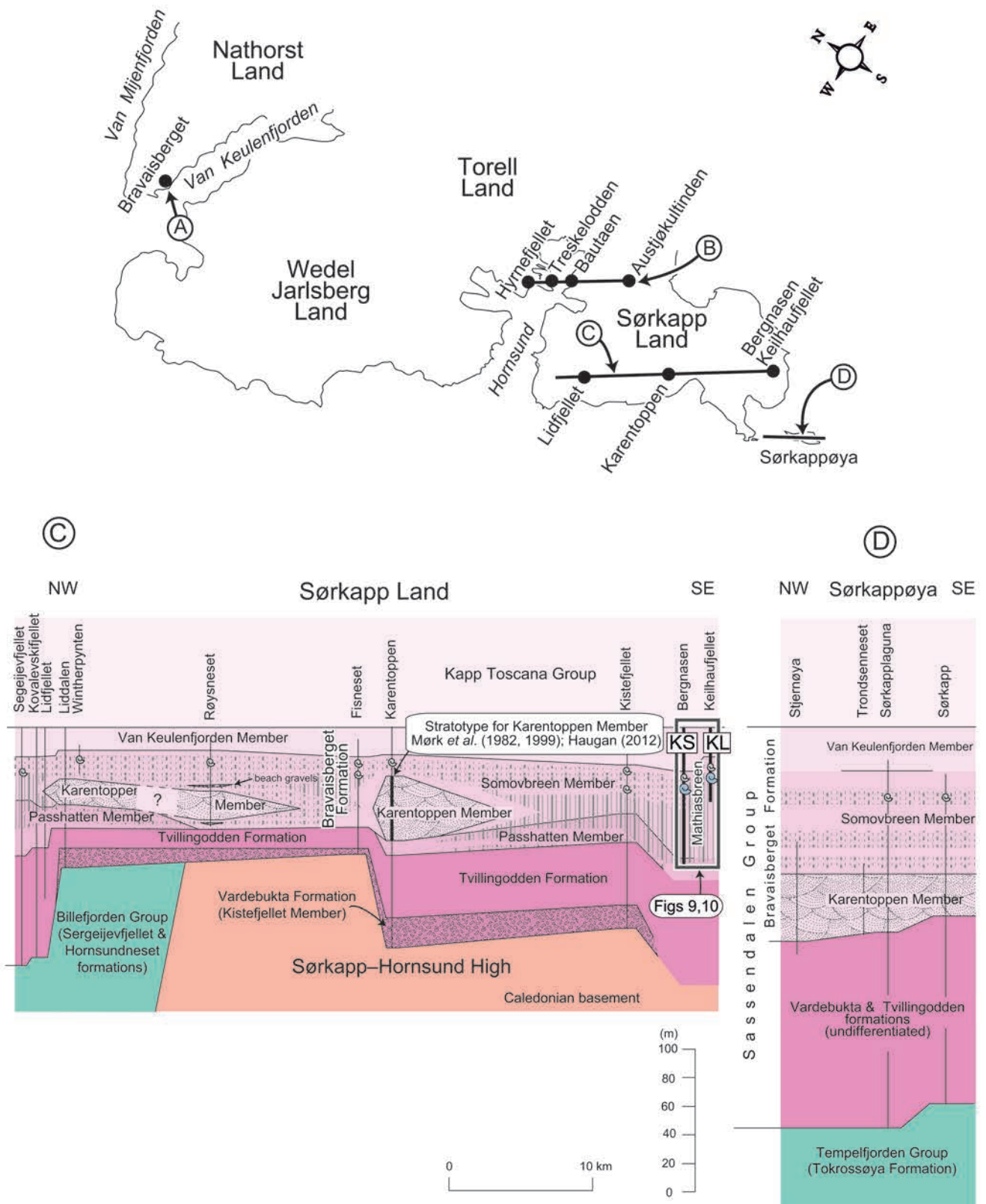
Fig. 3. Lithostratigraphy and facies of the Sassendalen Group in southern Spitsbergen. A. Van Keulenfjorden (Bravaisberget). B. Inner Hornsund and NE Sørkapp Land. C. Western coast of Sørkapp Land. D. Sørkappøya and Sjørnøya. For further explanation, see text.
