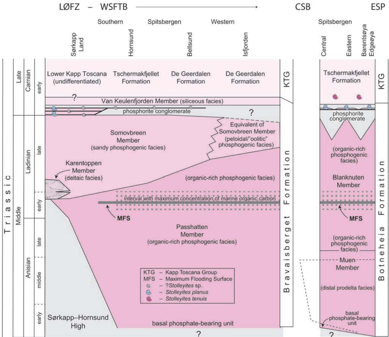
Fig. 14. Stratigraphic scheme of the Bravaisberget Formation of southern and western Spitsbergen and its suggested correlation with the Botneheia Formation of central and eastern Spitsbergen and eastern Svalbard. LØFZ – Lidfjellet-Øyrlandsodden Fold Zone; WSFTB – West Spitsbergen Fold-and-Thrust Belt; CSB – Central Spitsbergen Basin; ESP – Eastern Svalbard Platform (including central Spitsbergen). For further explanation, see text.
