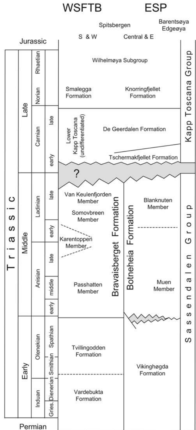
Fig. 2. The Triassic lithostratigraphic scheme of Svalbard after Nakrem and Mørk (1991), Mørk et al. (1999), Hounslow et al. (2007, 2008), and Hounslow and Nawrocki (2008), simplified. WSFTB – West Spitsbergen Fold-and-Thrust Belt (including the Lidfjellet-Øyrlandsodden Fold Zone); ESP – Eastern Svalbard Platform (including central Spitsbergen). For further explanation, see text.
