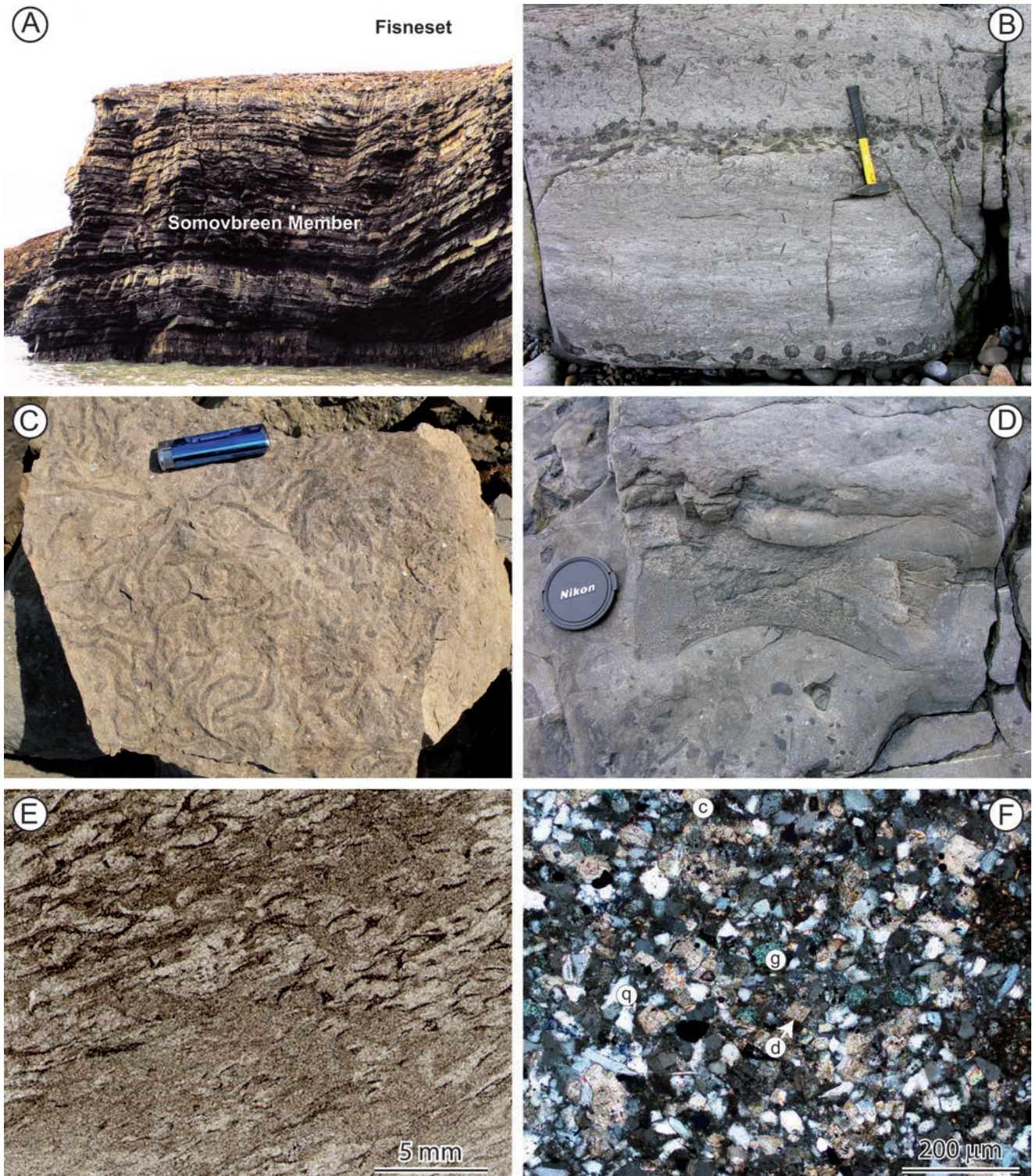
Fig. 5. Facies development of the Somovbreen Member in southern Spitsbergen. A. Succession of marine sandstones with siltstone/shale intercalations of the Somovbreen Member at Fiseset was deposited in front of deltaic sediments of the Karentoppen Member. The sandstone packages contain varying amounts of pristine and allochthonous phosphate nodules. B. Reworked horizons of allochthonous phosphate nodules and clasts in highly bioturbated sandstone of the Somovbreen Member at Røysneset. The sandstone contains common trace fossil Skolithos . C. Taenidium on a surface parallel to bedding in fine-grained sandstone of the Somovbreen Member at Keilhaufjellet. D. Reptilian bone in phosphatic sandstone of the Somovbreen Member at Røysneset. E. Finely bioturbated nature of sandstone of the Somovbreen Member at Kistefjellet. Thin section photograph. Section perpendicular to bedding. F. Photomicrograph of very fine-grained sandstone of the Somovbreen Member at Wintherpynten. The sediment consists of quartz ( q ) and glauconite ( g ) grains cemented by calcitic sparite ( c ). Diagenetic dolomite rhombs ( d ) occur as subordinate cement. Transmitted-light microscopy, crossed nicols.
