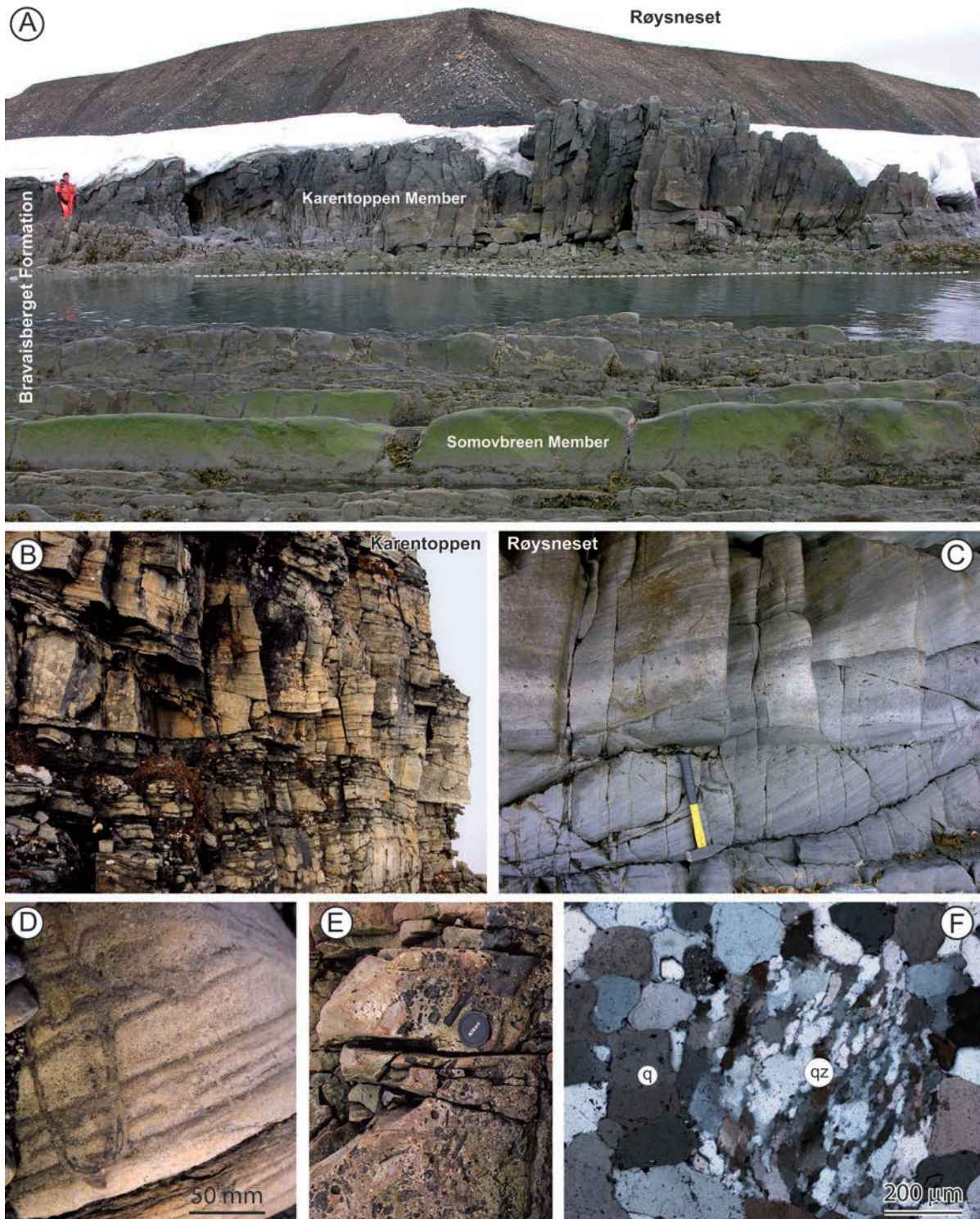
Fig. 6. Facies development of the Karentoppen Member in southern Spitsbergen. A. Medium- to coarse-grained sandstones filling delta distributary channel (Karentoppen Member) in the lower part of shallow marine sandstone succession of the Somovbreen Member at Røysneset. The Somovbreen Member contains in places lenses of beach gravelstone, composed of pebbles of different rocks of the Caledonian basement intermixed with allochthonous phosphate nodules and clasts. Note that the succession seen on the photo can be assessed during low tide of the sea. B. Part of a 30 m high cliff of the Karentoppen Member at Karentoppen showing medium- to coarse-grained sandstone lenses with tabular cross-bedding. Location of this cliff is shown in Fig. 1C. C. Medium- to coarse-grained sandstone lenses of the Karentoppen Member at Røysneset. The lenses show erosional boundaries, tabular cross-bedding with tangential foresets, and scattered land-plant detritus. Section perpendicular to bedding. D. Large Diplocraterion -like burrow that cuts lamina set of coarse-grained sandstone filling distributary channel at Sørkapplaguna on Sørkappøya. Section perpendicular to bedding. E. Land-plant detritus (black) in coarse-grained sandstone of the Karentoppen Member at Sørkapplaguna on Sørkappøya. Bedding plane. F. Photomicrograph of medium- to coarse-grained sandstone of the Karentoppen Member at Røysneset. The sandstone contains quartz ( q ) and quartzite ( qz ) grains, with subordinate admixture of other lithic grains. Transmitted-light microscopy, crossed nicols.
