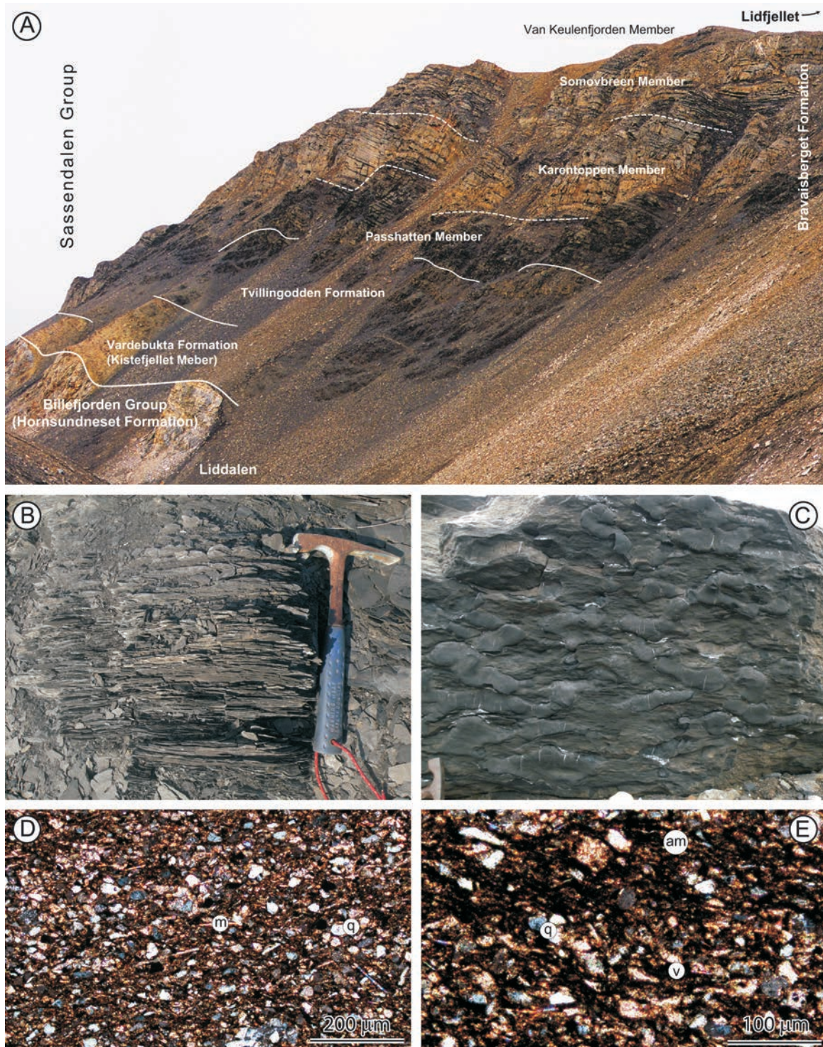
Fig. 4. Facies development of the Passhatten Member in southern Spitsbergen. A. Succession of the Sassendalen Group in Liddalen, NW Sørkapp Land. The succession belongs to the autochthonous part of the Lidfjellet tectonic structure (Lidfjellet-Øyrlandsodden Fold Zone), and records Triassic depositional history at northern margin of the Sørkapp-Hornsund High. The transgressive conglomerates and sandstones of the Kistefjellet Member (Vardebukta Formation) rest discordantly on quartzitic sandstones of the Carboniferous Hornsundneset Formation. They are overlain by laminated siltstones and shales of the Tvillingodden Formation. The Bravaisberget Formation is represented by the Passhatten, Karentoppen, Somovbreen, and Van Keulenfjorden members. The Passhatten Member comprises a cliff-forming black shale succession, reflecting organic-rich deposition at margin of the high before the input of coarse deltaic clastics of the Karentoppen Member. B. Non-laminated, fissile black shale of the Passhatten Member. Section perpendicular to bedding. Lidfjellet, NW slope. C. Flattened, phosphate-filled burrow system Thalassinoides in black shale of the Passhatten Member. Plane parallel to bedding. Lidfjellet, NW slope. D. Photomicrograph of black shale shown in (B). The shale contains quartz grains of the fine- to coarse-silt fractions ( q ) and detrital mica flakes ( m ) in a clay-rich matrix. E. Organic matter in the black shale is represented by seams of amorphous fraction ( am ) and vitrinite particles ( v ), preserved at an advanced stage of thermal alteration. Quartz grains ( q ) occur in the matrix. Lidfjellet, NW slope. (D, E) – transmitted-light microscopy, crossed nicols.
