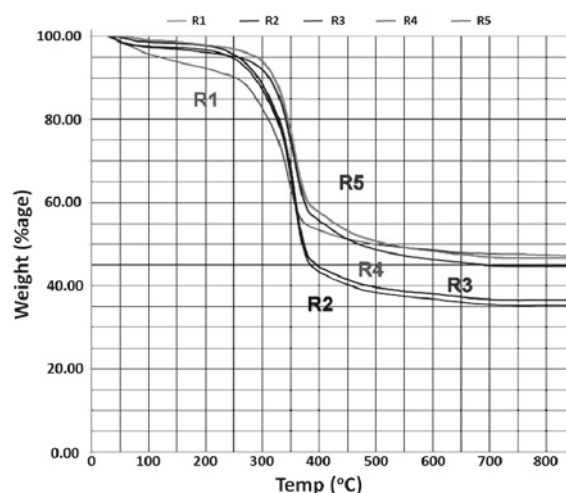
Figure 5. TGA graph for various RH samples
