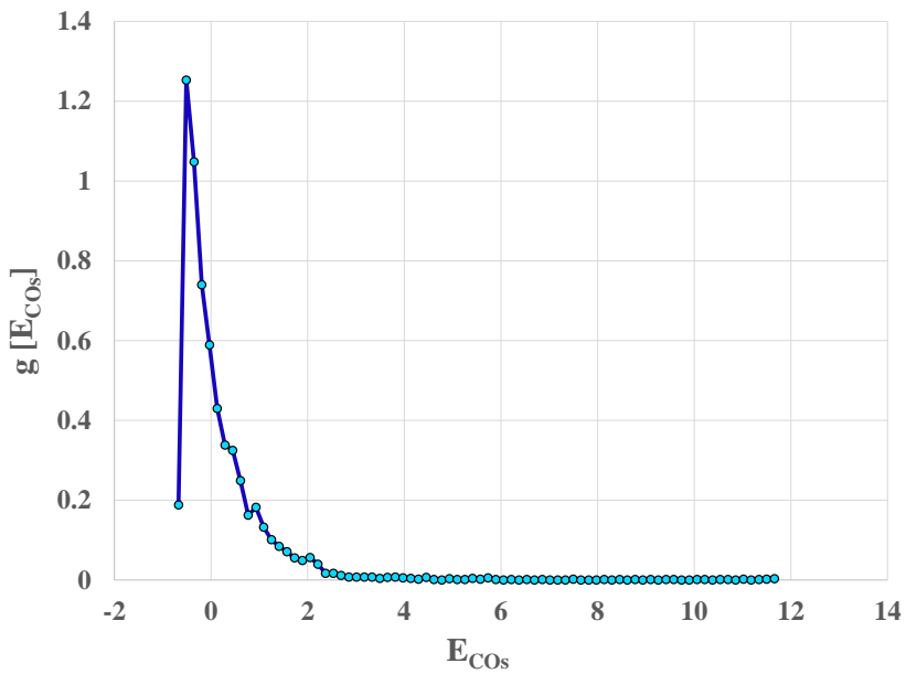
Fig. 28. Probability density – g of the process of the standardized intensity of CO emission – E_{COs}
