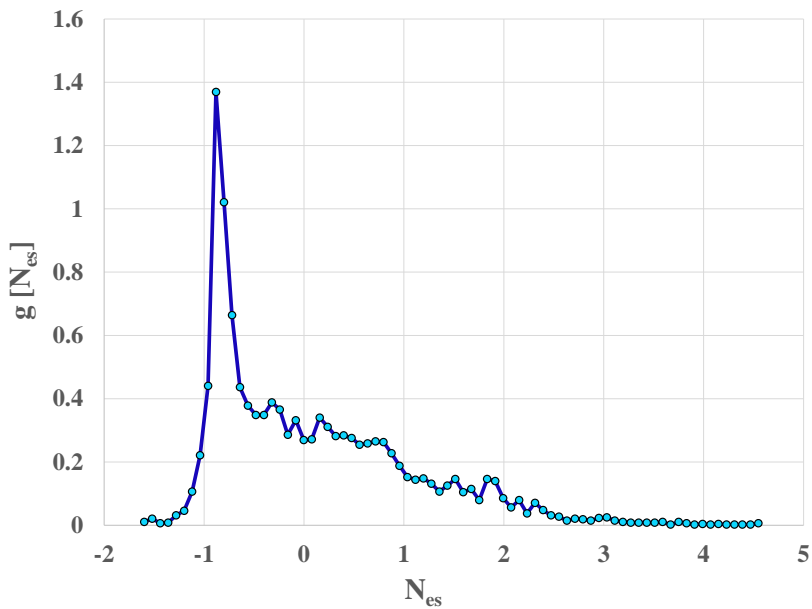
Fig. 27. Probability density – g of the process of the standardized useful power of a car engine – N_{es}
