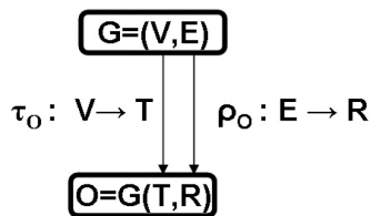
Fig. 2. Mapping of Vertices and Edges
