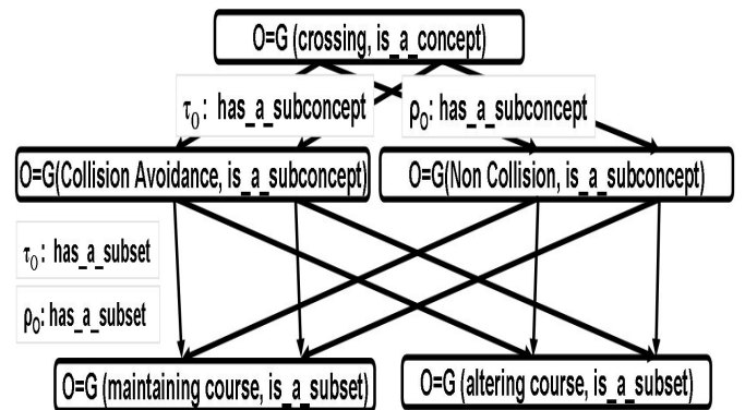
Fig. 8. Ontologies under the concept crossing
