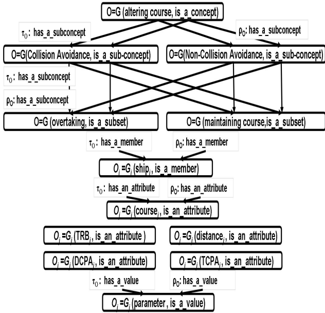
Fig. 9. Ontologies describing the concept altering course
