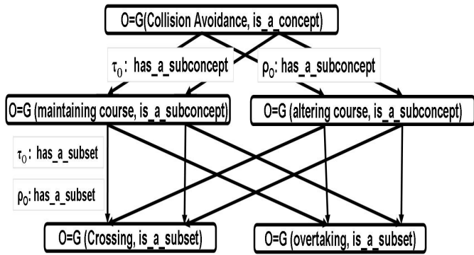
Fig. 3. Ontologies under the concept collision avoidance
