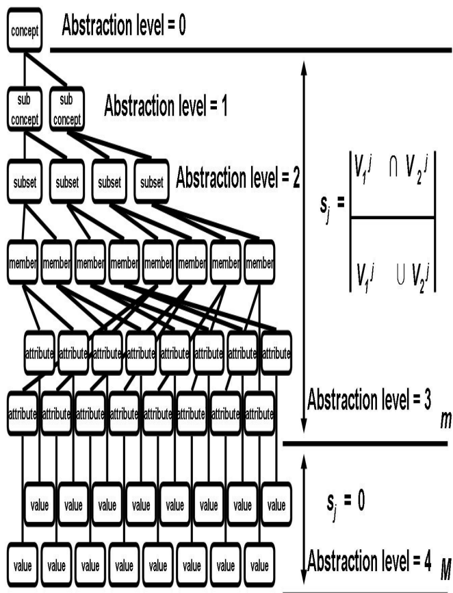
Fig. 10. Solving similarity using abstraction levels
