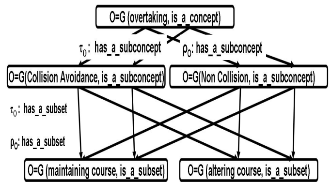
Fig. 7. Ontologies under the concept overtaking
