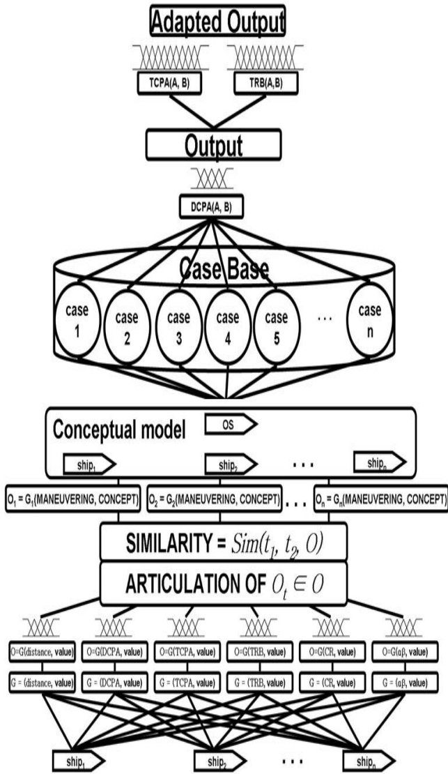
Fig. 12. Structure of building a conceptual model.
