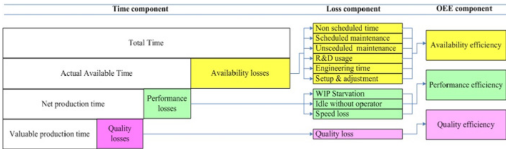
Fig. 2. OEE components based on Jeong and Phillips' concept (Jeong & Phillips, 2001)
