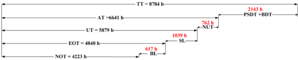
Fig. 6. Year-wise variations in time and losses (h) for the dragline under study
