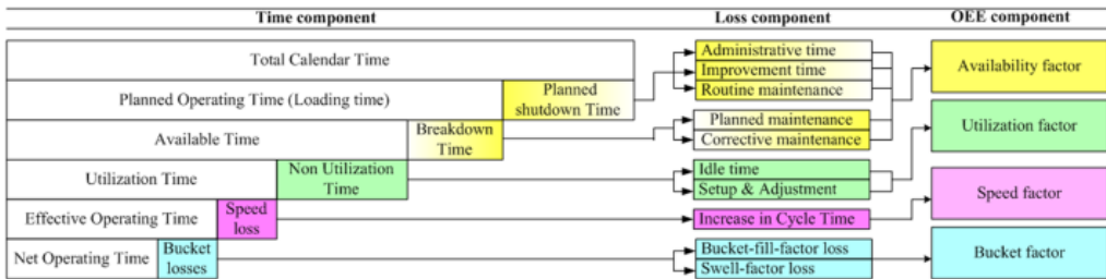
Fig. 4. OEE components of BELT equipment
