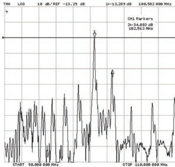
Fig. 8. Amplitude response of sensor with filter.
