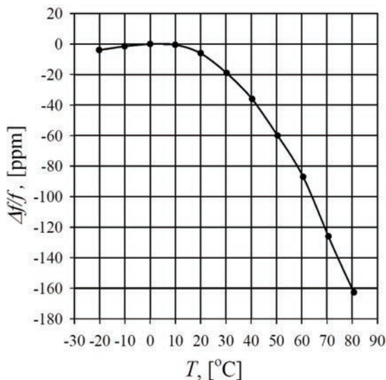
Fig. 9. Relative frequency changes against temperature.
