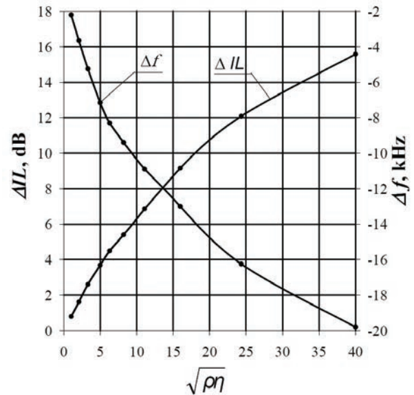
Fig. 10. Insertion loss ( \Delta IL ) and frequency ( \Delta f ) changes against \sqrt{\rho\eta} .
