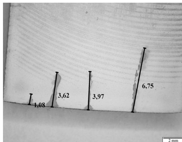
Fig. 5. The surface of the examined cast iron specimen after 1000 cycles of heating up to the 600°C and the subsequent water cooling; the micro-cracks shown in the photo are described with their respective length values (in millimetres) [17]
