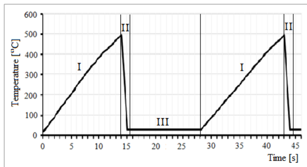
Fig. 4. An exemplary profile of heating and cooling of a single test part of a specimen; I – induction heating, II – rotation of the specimen and submersion in water, III – water cooling
