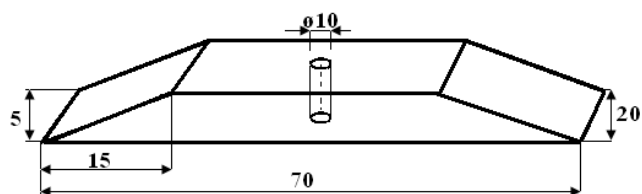
Fig. 3. The shape and dimensions of a specimen used for examination of thermal shock resistance of the material; the central opening was used for mounting the specimen on a special holder integrated with the rotational boom arm
