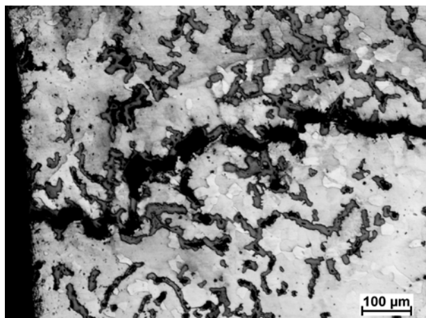
Fig. 6. Microstructure of the vermicular cast iron with the revealed micro-crack propagating from the edge towards the core of the specimen; the specimen underwent 200 cycles of heating up to the temperature of 500°C and the subsequent cooling [17]
