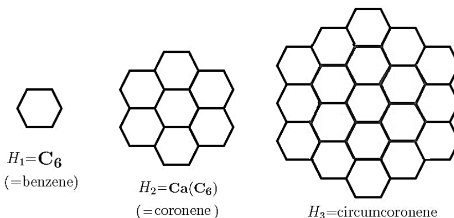
Figure 1. Three first members of Circumcoronene Homologous Series of Benzenoid: H_1 = \textit{benzene} , H_2 = \textit{coronene} and H_3 = \textit{circumcoronene} [18-26].
