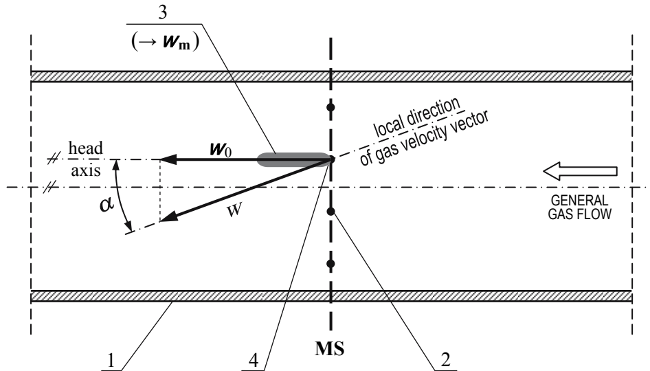
Fig. 3. Schematic illustration of the issue of accuracy of axial velocity measurement in situation of local gas flow deviation and setting the velocity sensor coaxially with the conduit, with gas velocity variation exclusively in plane parallel to conduit wall 1 – conduit wall, 2 – measurement points, 3 – velocity sensor head, 4 – sensor nose, MS – measuring section
