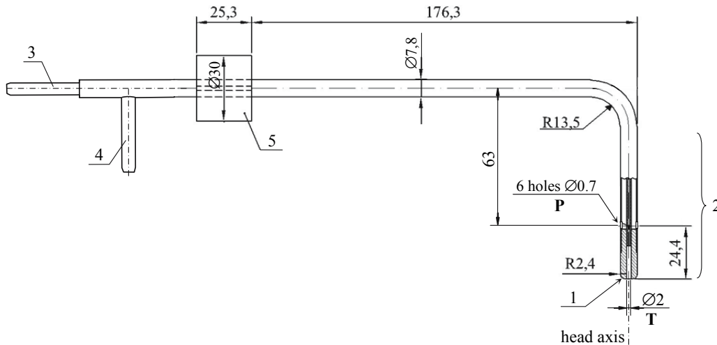
Fig. 6. L-type impact-pressure tube under test
