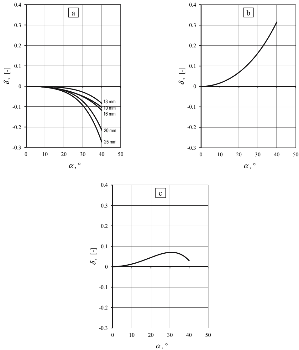
Fig. 14. Relative error \delta of determination of axial velocity w_0 in situation of deviated local gas flow and setting the velocity sensor coaxially with the conduit for:
