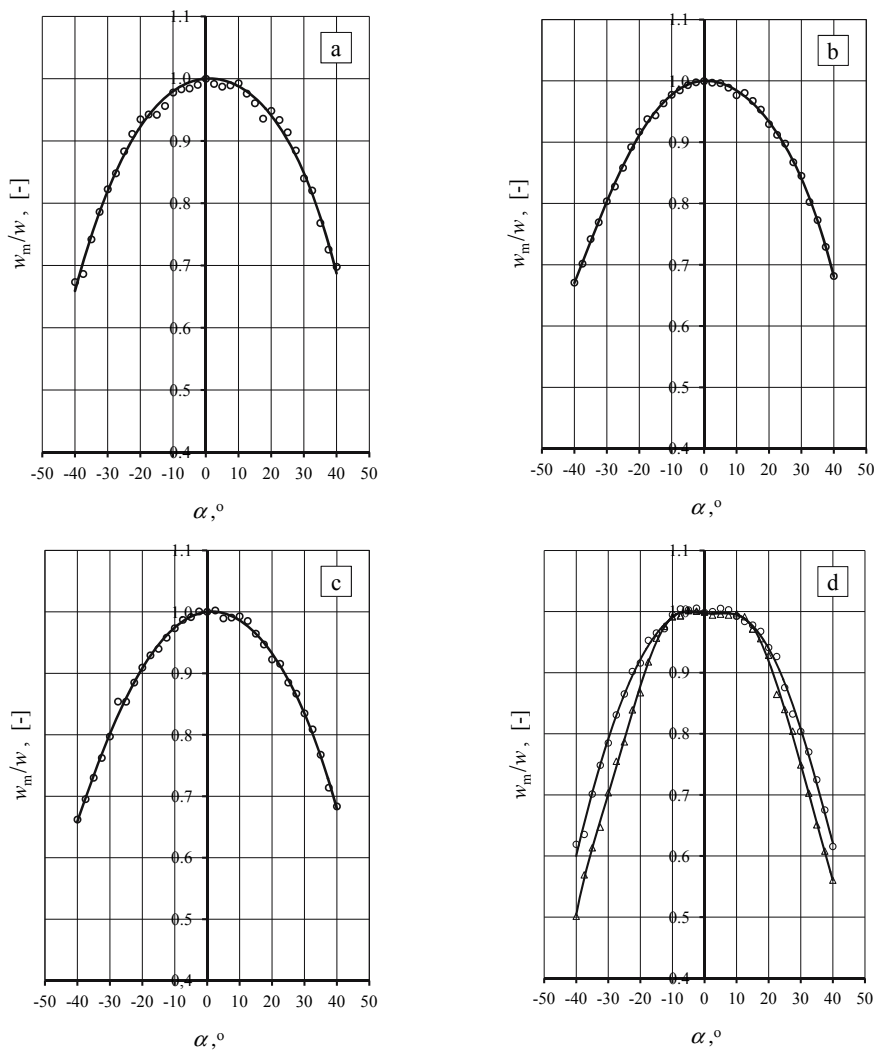
Fig. 10. Relative measured velocity w_m/w in relation to angle \alpha for: a – the probe with the aspiration nozzle d_a = 16 mm and w = 7.7 m/s, at \epsilon = 10\% b – the probe with the aspiration nozzle d_a = 16 mm and w = 10.9 m/s, at \epsilon = 10\% c – the probe with the aspiration nozzle d_a = 16 mm and w = 13.9 m/s, at \epsilon = 10\% d – the probe with the aspiration nozzle d_a = 20 mm and w = 6.8\div 6.9 m/s, at \epsilon = 0.8\% ( \Delta ) and \epsilon = 10\% (O)
