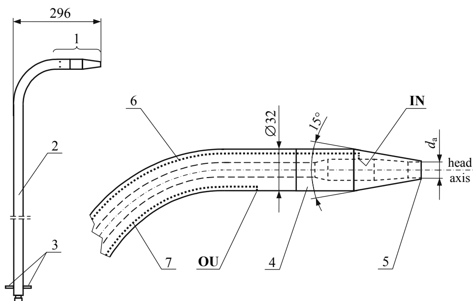
Fig. 4. Zero pressure probe under test
