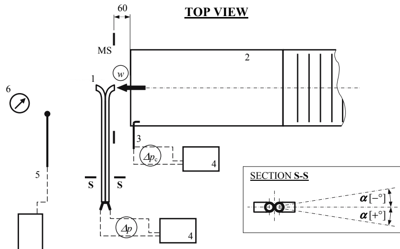
Fig. 9. System of measuring gas velocity with the S-type and L-type impact-pressure tubes under test 1 – S- or L-type tube (here: S-type as an example), 2 – discharging section of the wind tunnel (with turbulizers), 3 – control microtube, 4 – differential pressure micromanometer, 5 – temperature and absolute pressure meter, 6 – hair hygrometer, MS – measuring section; (drawing not to scale)
