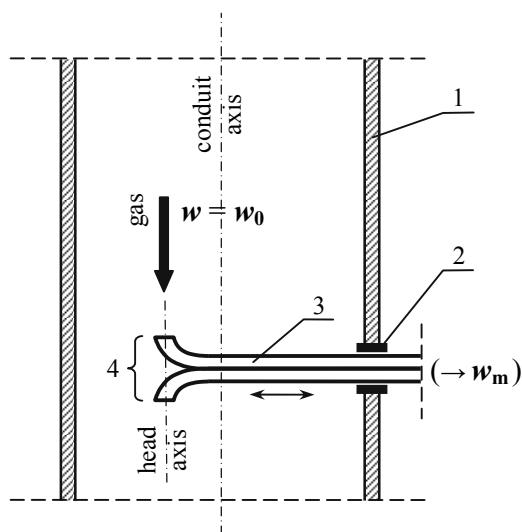
Fig. 1. Schematic illustration of the ideal measurement situation: of gas flow parallel to the axis and the wall of the conduit
