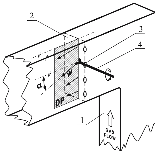
Fig. 2. Case of variation of gas velocity vector in planes parallel to conduit wall
