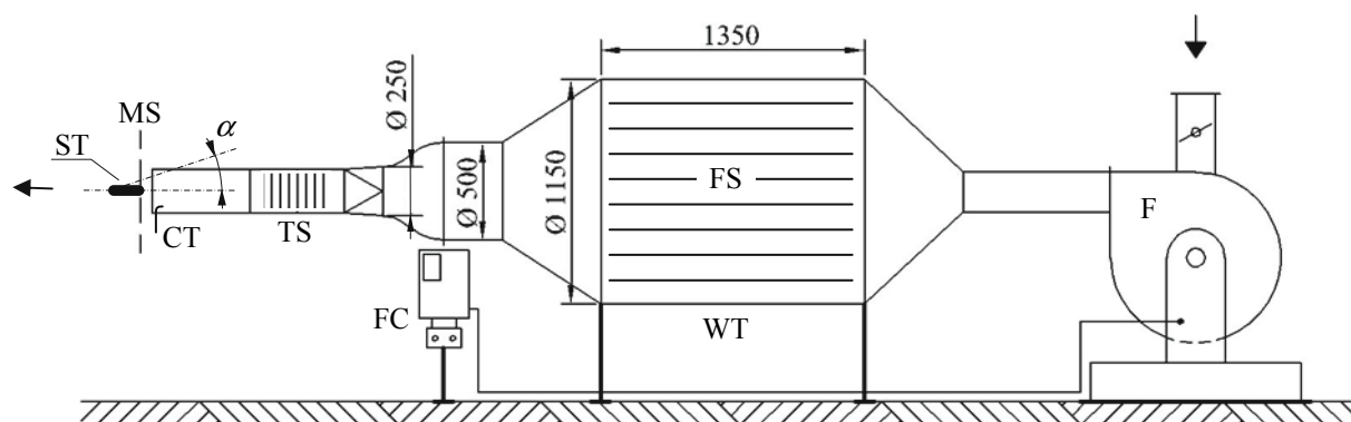
Fig. 7. General scheme of the test stand (in front view)
