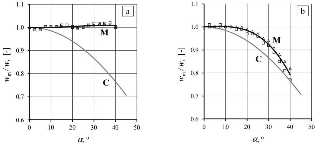
Fig. 13. Relative measured velocity w_m/w in relation to one-sided angle \alpha (or directional sensitivity) against a background of relative actual axial velocity (or \cos\alpha ) for the impact-pressure tubes
