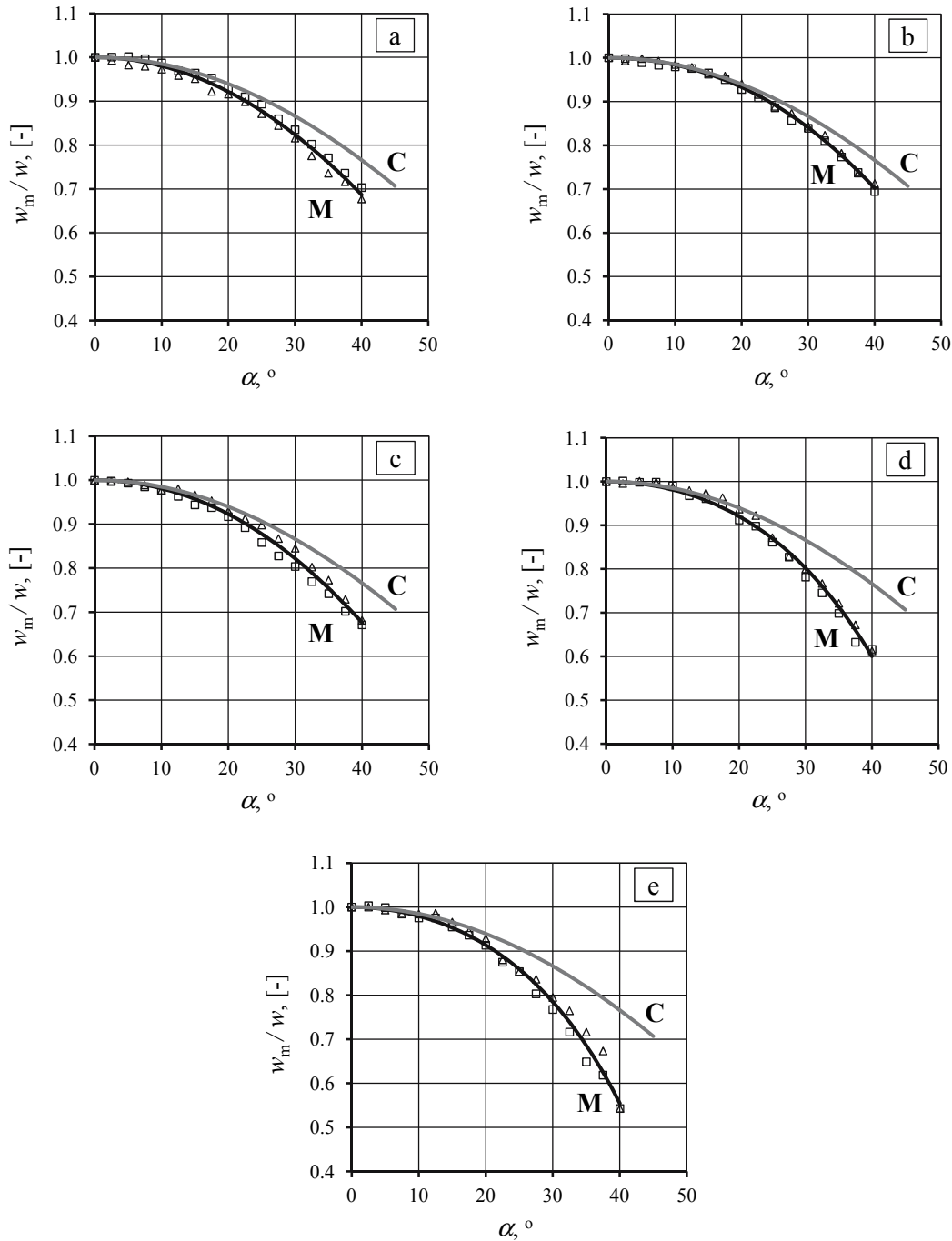
Fig. 12. Relative measured velocity w_m/w in relation to one-sided angle \alpha (or directional sensitivity) against a background of relative actual axial velocity (or \cos\alpha ) for the P-10ZA dust sampler probe
