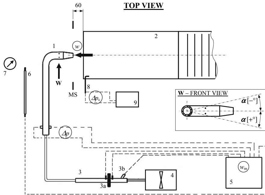
Fig. 8. System of measuring gas velocity with the zero pressure dust probe under test
