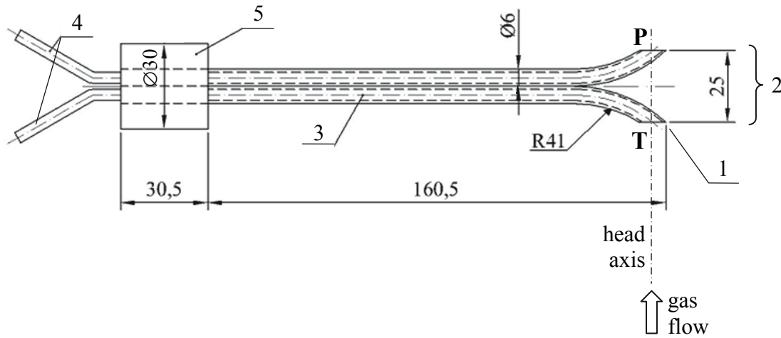
Fig. 5. S-type impact-pressure tube under test
