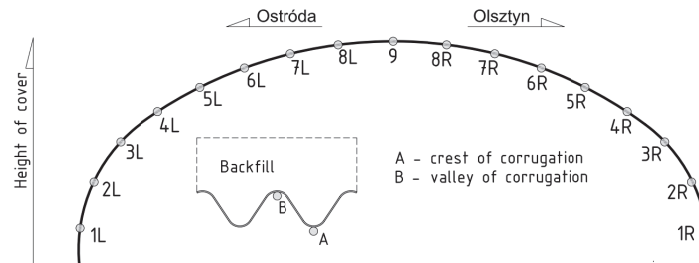
Figure 6. Locations of the strain gauges
