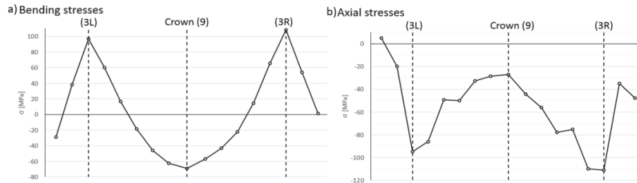
Figure 8. Distribution of a) bending stresses and b) axial stresses for the height of backfill equal to 6,3 m over the top of the foundation.
