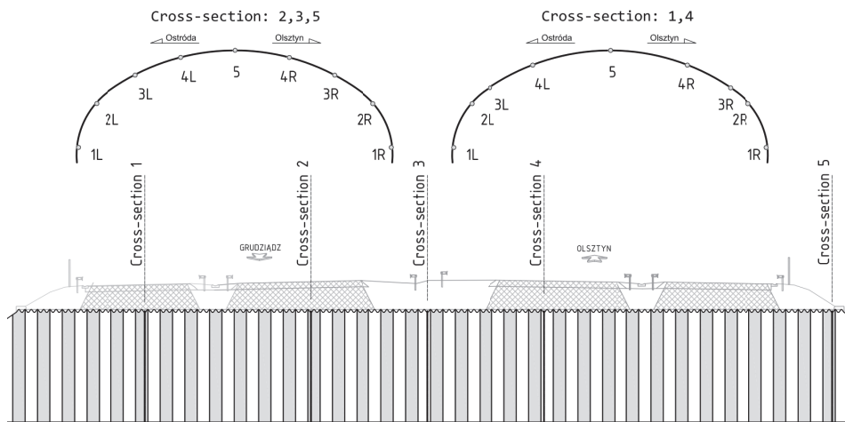
Figure 5. Locations of the optical prism
