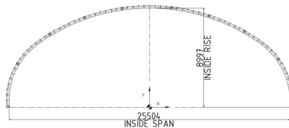
Figure 1. Structure geometry (Cross section)
