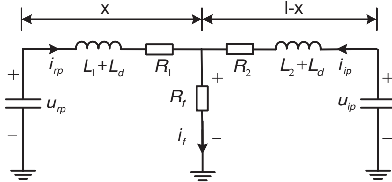
Fig. 6. Equivalent circuit of positive pole-to-ground fault
