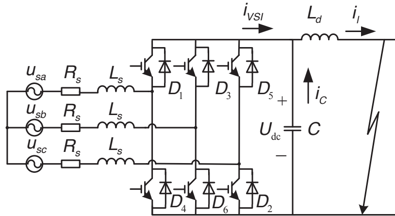
Fig. 2. Equivalent circuit of pole-to-pole fault
