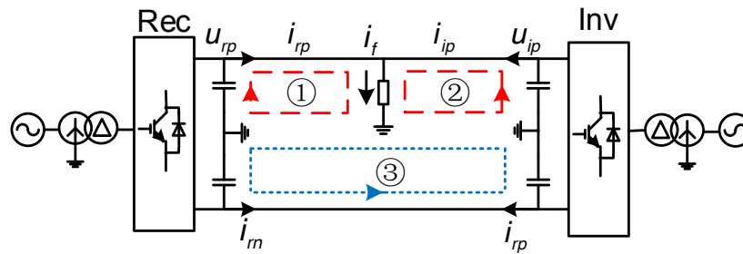
Fig. 5. Circuit loop of positive grounding fault
