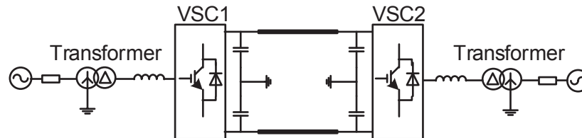
Fig. 1. Typical earthing mode of two-terminal VSC-HVDC
