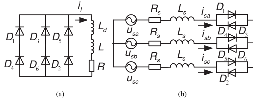
Fig. 4. Equivalent circuit of diode freewheel stage: DC side (a); AC side (b)
