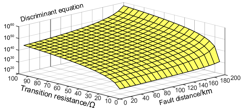
Fig. A1. The relationship between discriminant equation, fault distance and transition resistance
