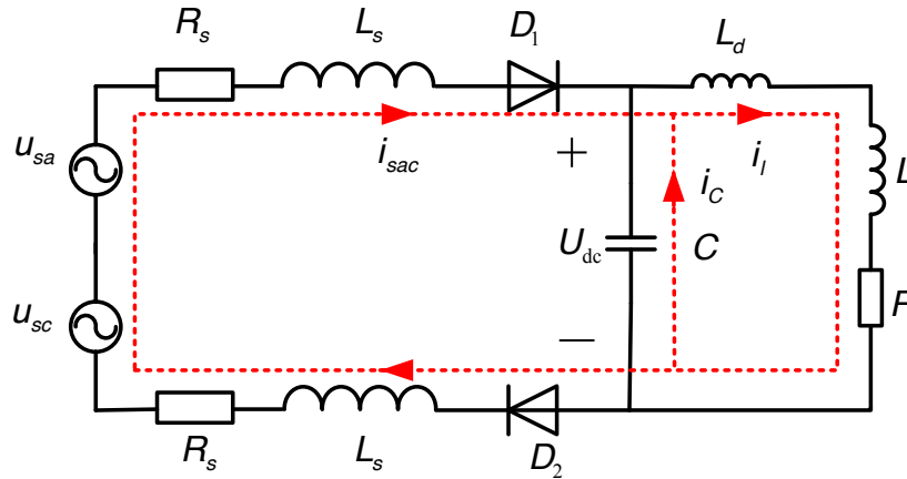
Fig. 3. Equivalent circuit diagram of D_1, D_2 conduction
