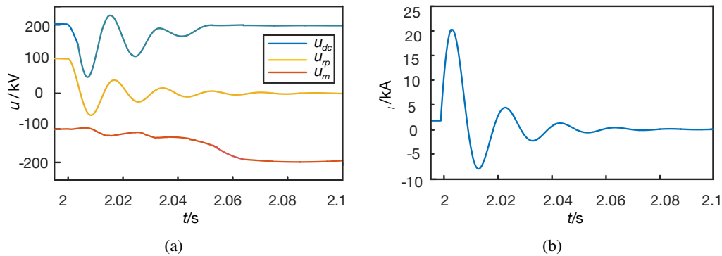
Fig. 8. pole-to-ground fault voltages and current on rectifier side: voltages (a); DC fault current (b)
