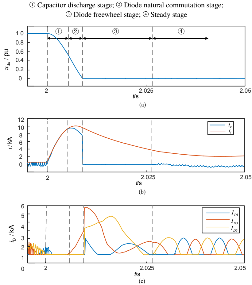
Fig. 7. Oscillogram of pole-to-pole fault transient stages: DC voltage on rectifier side (a); currents in fault line and capacitor on rectifier side (b); currents in common-anode diodes (c)
