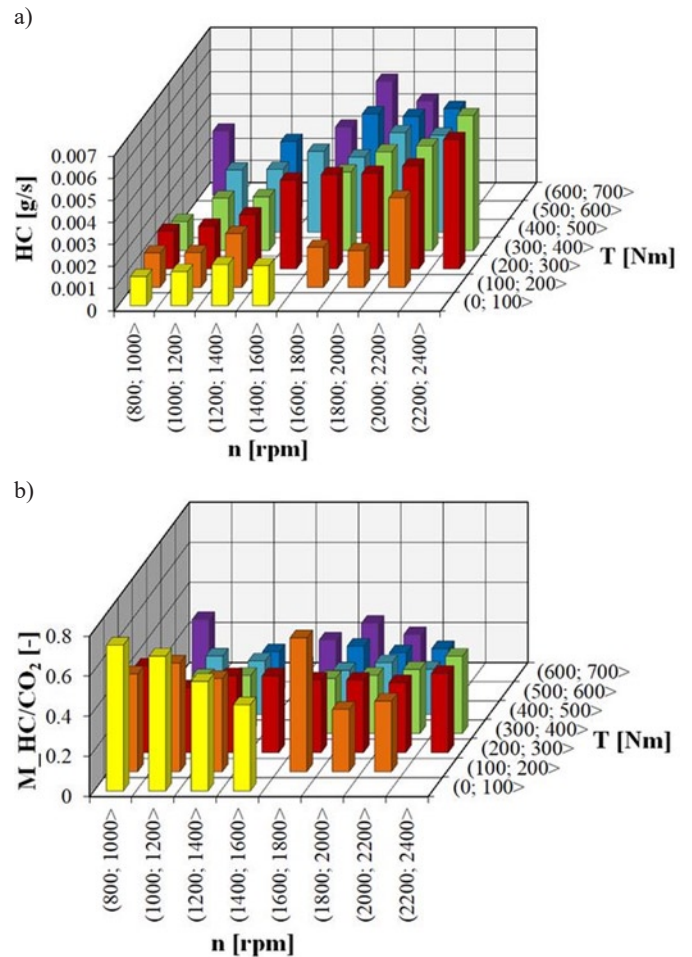
Fig. 8. Characteristics of a) second HC emission rate; b) HC emissivity in the torque ranges of the engine speed
