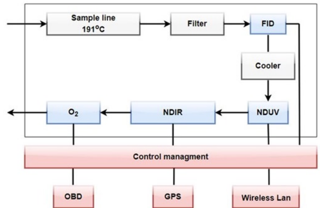
Fig. 3. Diagram of operation of PEMS- SEMTECH DS apparatus [23]
