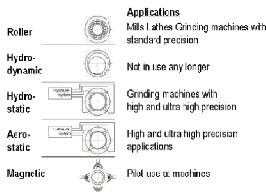
Fig. 5 Bearings of main spindles and their application
