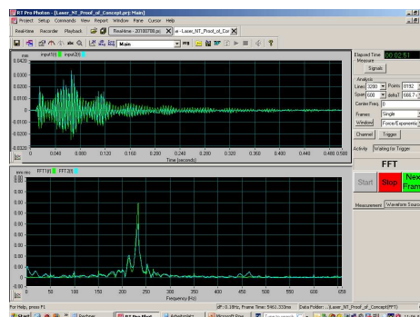
Fig. 8. Compliance of laser vibrometer (green) and LaserControl (blue)
