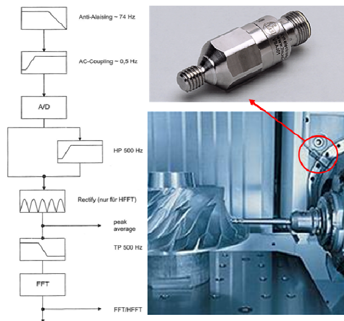
Fig. 4 Scheme for demodulating vibration data for bearing condition monitoring (left). Condition monitoring with a capacitive acceleration sensor (right)
