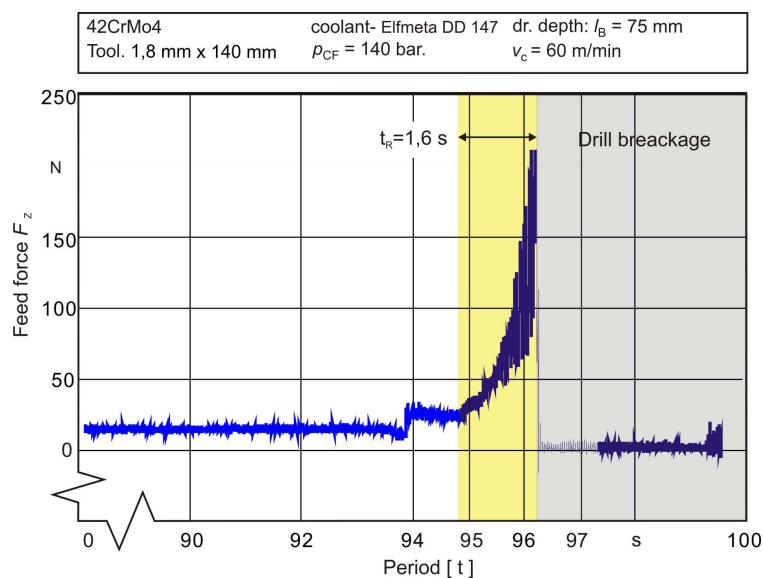
Fig. 13. Forward feeding force for transiting different materials with time to react before rupture of drill
