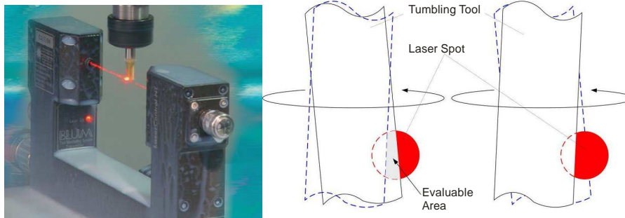
Fig. 6. Sensor Blum Novotest "LaserControl" for detecting tool
