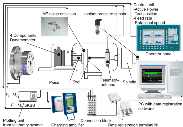
Fig. 12. Scheme of the measuring system used
