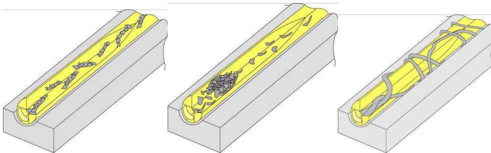
Fig. 11. Chip removal in stationary process, processes disturbance of chip entanglement and clogging (left to right)
