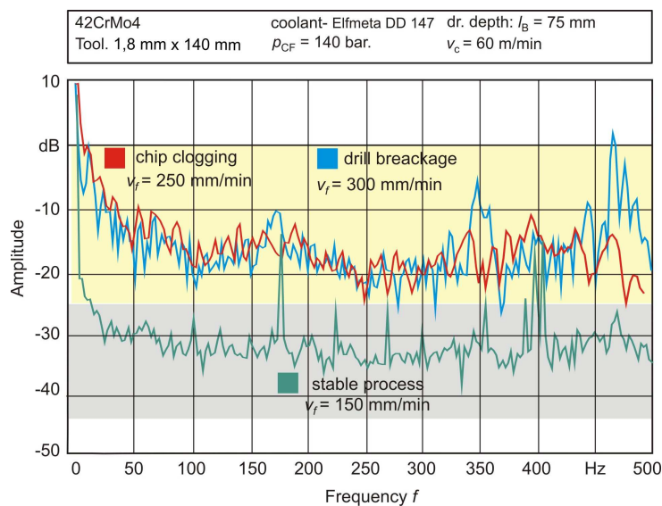
Fig. 14. Transformed feed force signals in stable and unstable gun drilling processes
