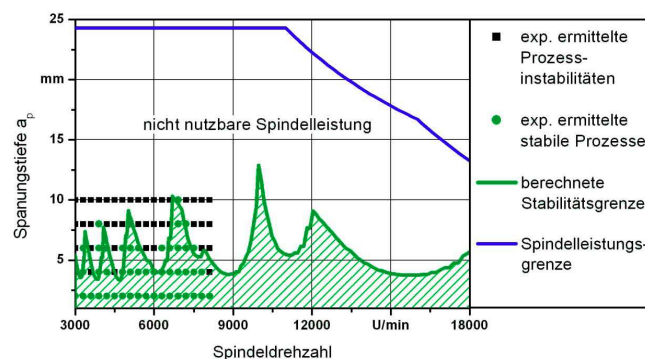
Fig. 3. Limitations of the usability of the main spindle's performance due to dynamic stiffness [2]
