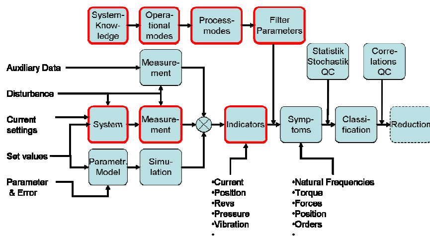
Fig. 1. Structure of process monitoring
