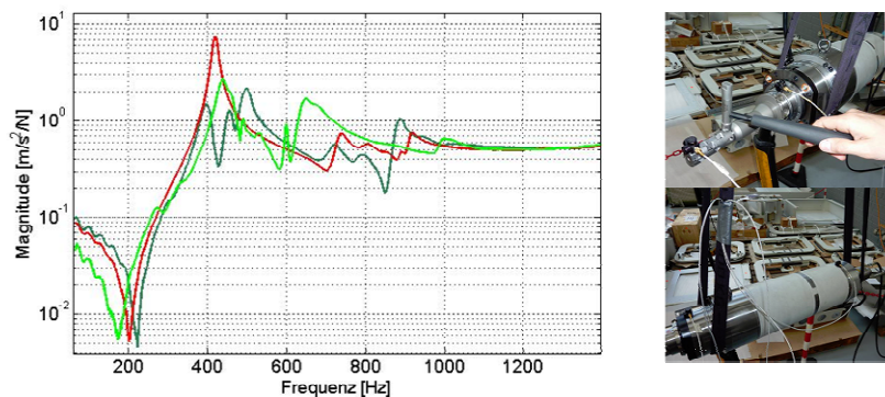
Fig. 9. Frequency response of a main spindle at the casing (green) and at the tool (red)
