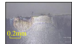
Test piece No.1, Removal volume 605473 \text{ mm}^3
