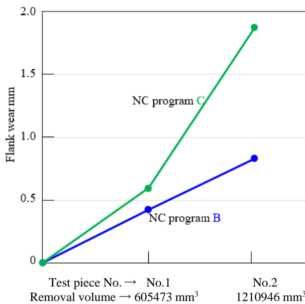
Fig. 10 Tool life test results for experiments using NC program B and C.
