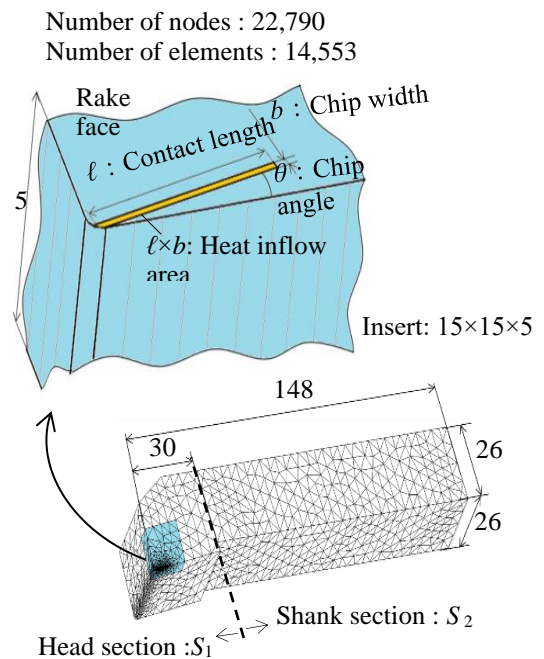
Fig. 1. FEM thermal analysis model of the insert for calculating the training data of the neural network. Heat flow areas and its specifications are shown in the figures
