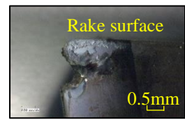
(a) NC program A before correct (Spindle speed 1200 \text{ min}^{-1} , At workpiece diameter \phi 68 and removal volume 253338 \text{ mm}^3 )
