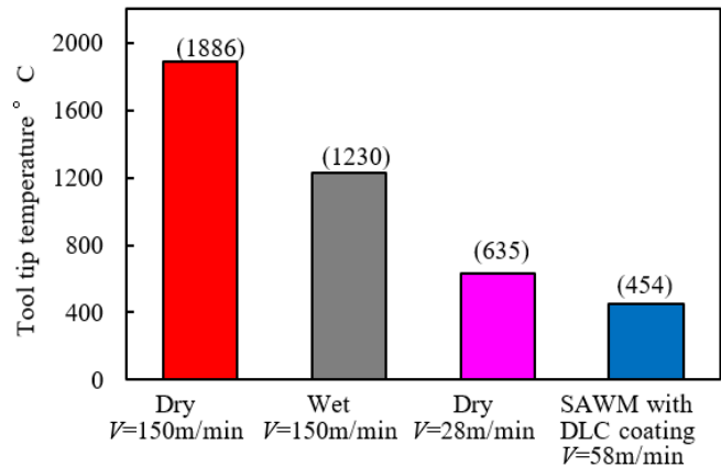
Fig. 4. Experimental results for the tool tip temp. Countermeasure using the proposed program was a success. Because the optimum cutting speeds for the free-cutting temperature of the insert. were calculated by the program
