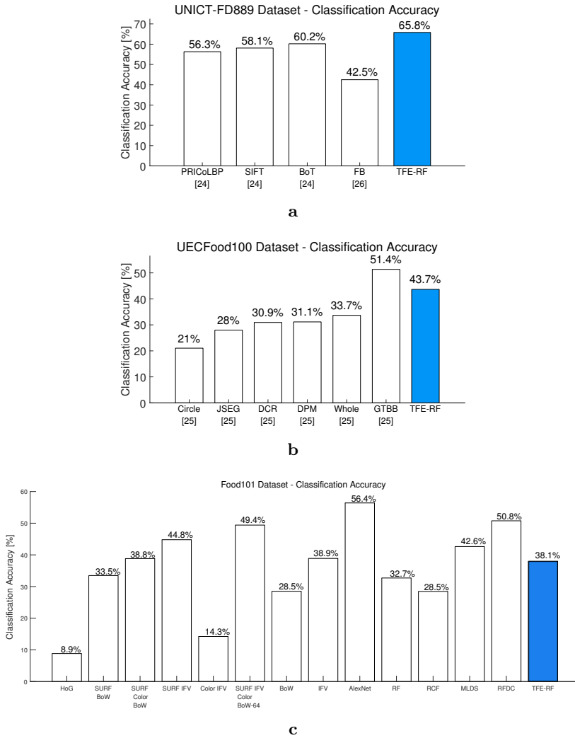
Fig. 11: Performance of the proposed TFE-RF approach is compared to state-of-the-art ones. Results are shown for the (a) UNICT-FD889, (b) UECFood100, and (c) Food101 datasets.
