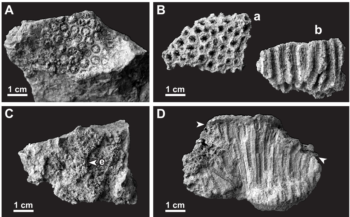
Fig. 4. Heliastraea defrancei (Milne-Edwards & Haime) from the upper Badenian Ternopil Beds of western Ukraine. A. Natural imprint of the upper surface of a colony (specimen no. MWGUW ZI/81/024 from Sakhkamin). B. Fragment of a well-preserved colony, a – top view, b – side view (specimen no. MWGUW ZI/81/005 from Saryi Zbarazh). C. Natural imprint of the upper surface of colony, “e” – “ Entobia balls” – moulds of borings of clionid sponges (specimen no. MWGUW ZI/81/021 from Sakhkamin). D. Fragment of a colony with encrustations of coralline-algae, resulting in temporal halt in coral development (specimen no. MWGUW ZI/81/050a from Maksymivka).
