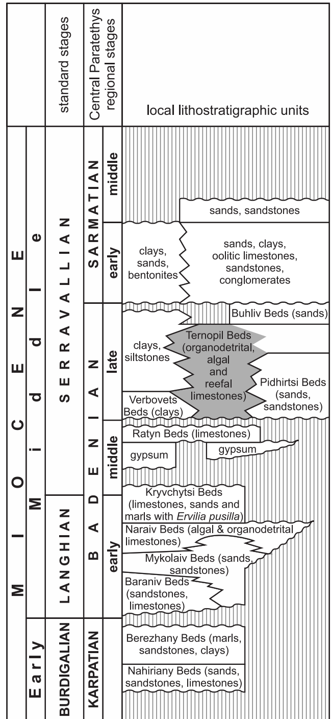
Fig. 2. Position of the upper Badenian coral-bearing deposits of Ternopil Beds studied in western Ukraine within the regional and standard zonations schemes (compiled from: Andreyeva-Grigovich et al. , 1997; Górká et al. , 2012; Radwański et al. , 2014).
