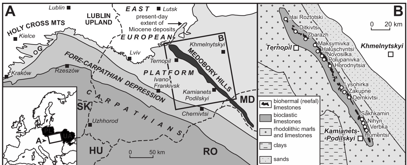
Fig. 1. Location of coral-bearing sites studied in the Medobory Hills in western Ukraine. A. Location within Europe, in relation to Poland/Ukraine border. G – the site of Grobie in Poland, where an early Badenian coral-reef was recorded. B. Detailed map, showing the location of sites and extent of lithofacies in the Medobory Hills and their vicinity during the late Badenian (after Korolyuk, 1952; Kudrin, 1966; Górka et al. , 2012; changed).
