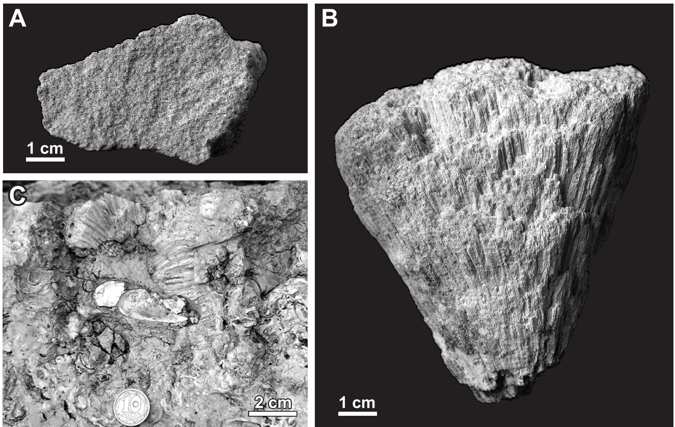
Fig. 5. Siderastraea italica (Defrance) from the upper Badenian Ternopil Beds of western Ukraine. A. Fragment of a well-preserved, massive colony, top view (specimen no. MWGUW ZI/81/029a from Zakupne). B. Fragment of a large, massive colony, side view (specimen No. MWGUW ZI/81/002 from Maksymivka). C. Fragment of a large colony with boring and shell of Lithophaga sp. (specimen no. MWGUW ZI/81/004 from Humentsi, field photograph).
