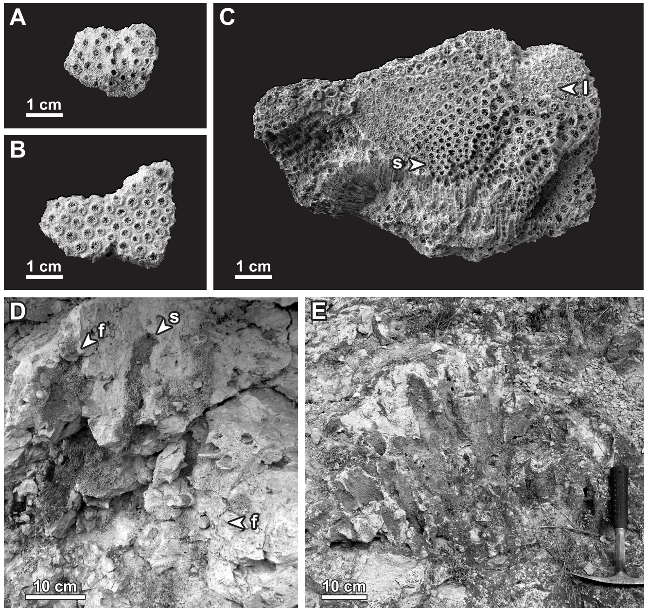
Fig. 3. Tarbellastraea reussiana (Milne-Edwards & Haime) from the upper Badenian Ternopil Beds of western Ukraine. A. Fragment of colony with small calices and wide inter-calice spaces, top view (specimen no. MWGUW ZI/81/019 from Sakhkamin). B. Fragment of colony with wide calices and small inter-calice spaces, top view (specimen no. MWGUW ZI/81/020 from Sakhkamin). C. Fragment of colony with calices differing in size, top view (specimen no. MWGUW ZI/81/007 from Humentsi). D. Natural imprint of colony made up of flat branches (“f”) passing upwards into vertical (“s”) sticks (field photo from Demkivtsi). E. Natural imprint of bush-shaped colony made up of large sticks (field photo from Demkivtsi).
