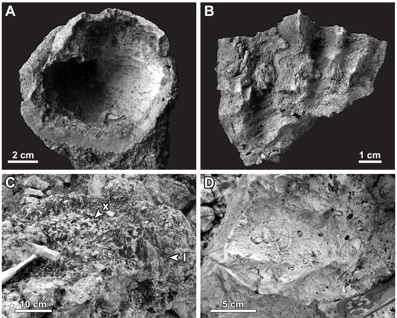
Fig. 6. Porites vindobonarum prima Kühn in Felix from the upper Badenian Ternopil Beds of western Ukraine. A. Spheroidal colony, partially neomorphised, internal part completely dissolved (specimen no. MWGUW ZI/81/010 from Nihyn). B. Natural imprint of a branching “organ pipe” colony, side view (specimen no. MWGUW ZI/81/018 from Sakhkamin). C. Large branching “organ pipe” colony, “x” – cross-sections, “l” – longitudinal sections (field photograph from Sakhkamin). D. Partially neomorphised massive colony with numerous borings of bivalves, mainly Lithophaga sp. (field photograph from Zakupne).
