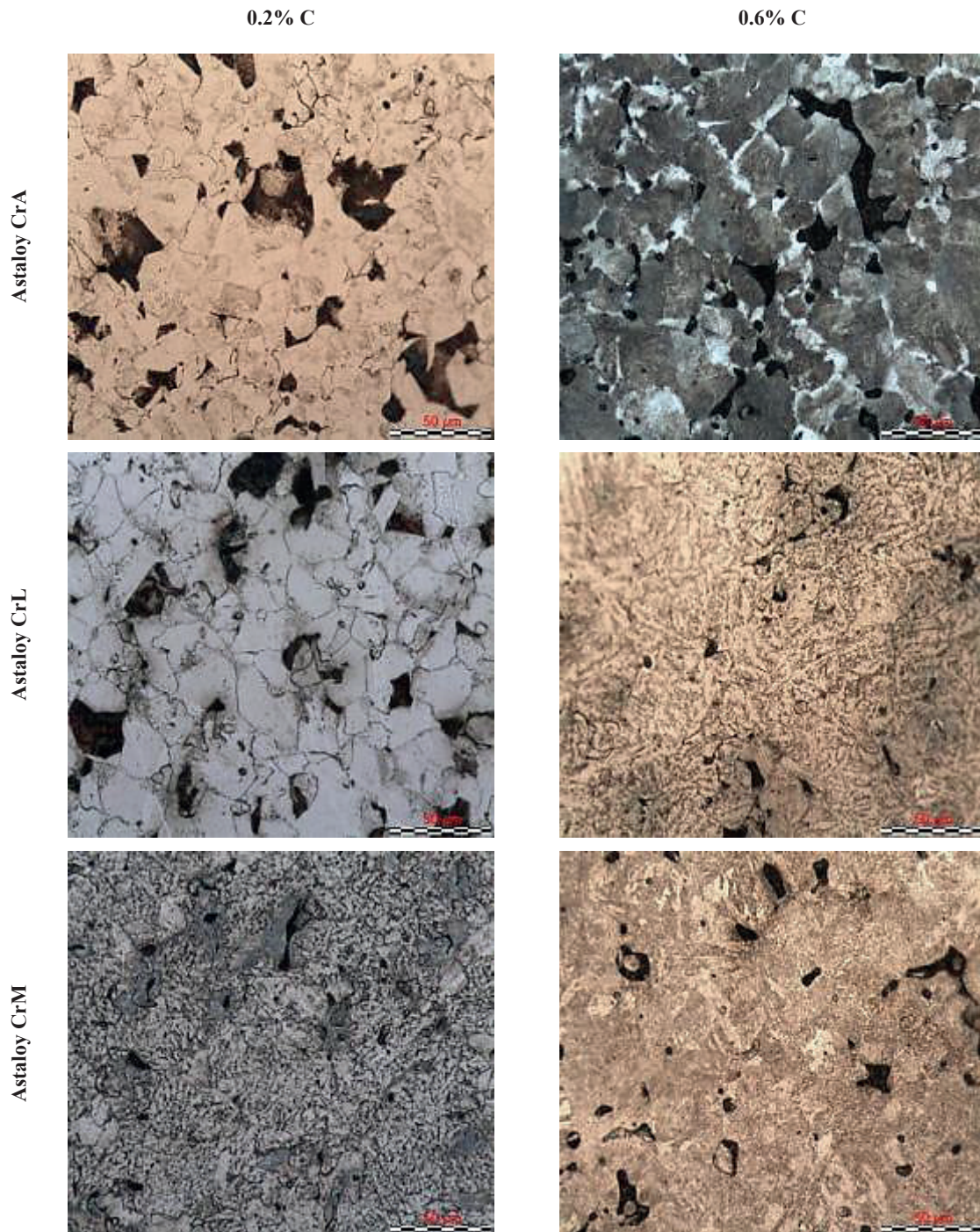
Fig 3 The characteristic microstructures of steel sintered at 1250°C (marker 50 \mu\text{m} )
