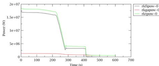
Fig. 21. Power generated in the fuel assembly.
