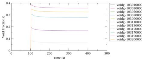
Fig. 12. Void fraction.
