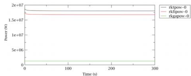
Fig. 9. Power generated in the fuel assembly.
