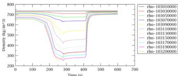
Fig. 19. Moderator density.
