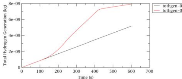
Fig. 22. Hydrogen production.
