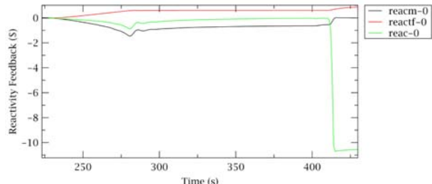
Fig. 20. Reactivity feedbacks.
