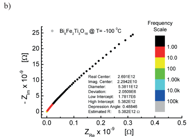
Fig. 5. Impedance diagrams in the complex Z''-Z' plane measured for \text{Bi}_6\text{Fe}_2\text{Ti}_3\text{O}_{18} ceramics at temperature T=0^\circ\text{C} (a), T=-100^\circ\text{C} (b); isotropic (a) and free scale (b) was used for data presentation
