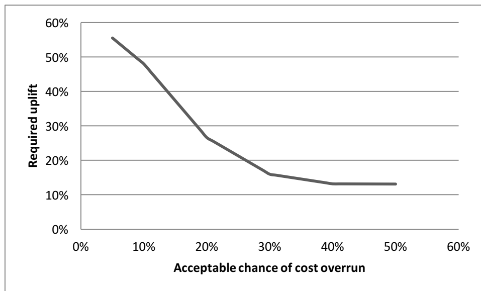
Fig. 8. Uplift as a function of the maximum acceptable level of risk for cost overrun – Fixed links (Contractors)
