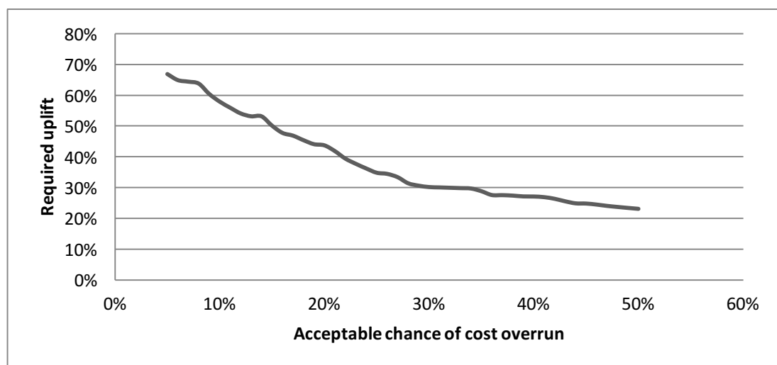
Fig. 6. Required uplift as a function of the maximum acceptable level of risk for cost overrun – Roads (contractors)
