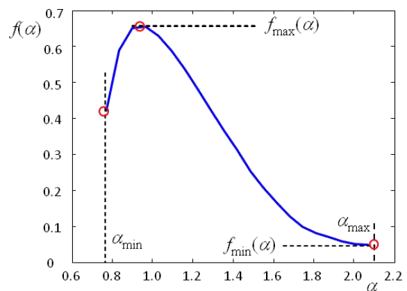
Fig. 1. Typical shape of MF spectrum.
