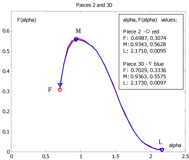
Fig. 3. MF spectra of the second pieces of the song Dancing Queen : 2 (ABBA) and 30 (MOVIE).
