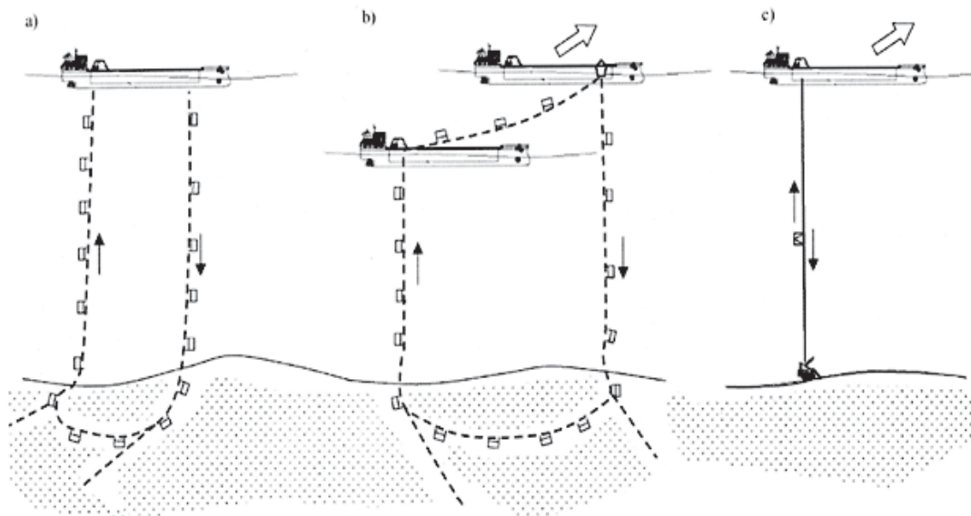
Fig. 13. Examples of mechanical extracting installments: a) Rope-container method with one ship (Japanese version); b) Rope-container methods with two chips (French version); c) Rope-container method with aggregate collecting concretions, source: Abramowski and Szelangiewicz, 2011
