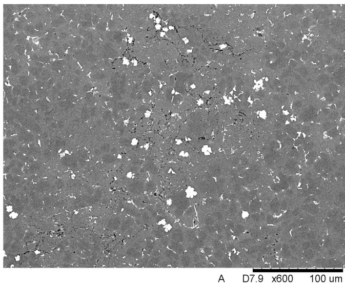
Fig. 5. View of cast F structure with shrinkage-gas microporosity, magnification: 600×
