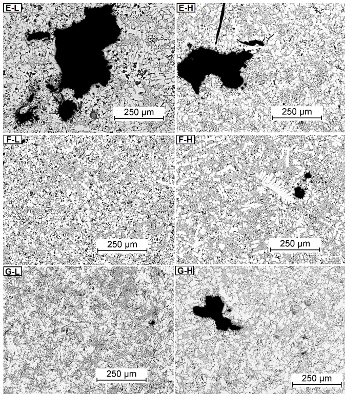
Fig. 4. View of samples' microstructure casts E-G, magnification: 50×, non-etched
