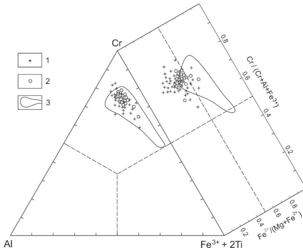
Fig. 2. The Al-Cr- \text{Fe}^{3+} - \text{Mg}/(\text{Mg} + \text{Fe}^{2+}) diagram of spinelides from the Inagli massif. 1, chromite intergrown with isoferroplatinum from the placer; 2, schlieren-veinlets chromitites in dunite; 3, the field of accessory chromian spinel (n=101 analyses) from dunite.
