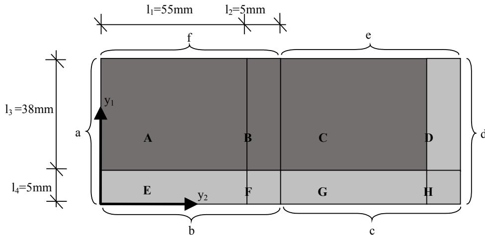
Fig. 1. Assumed geometry of periodic cell of masonry
