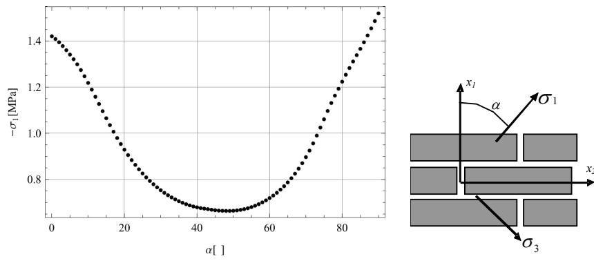
Fig. 3. Lower bound strength assessment for masonry. Directional uniaxial compression
