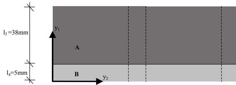
Fig. 8. Geometry of layered microstructure considered
