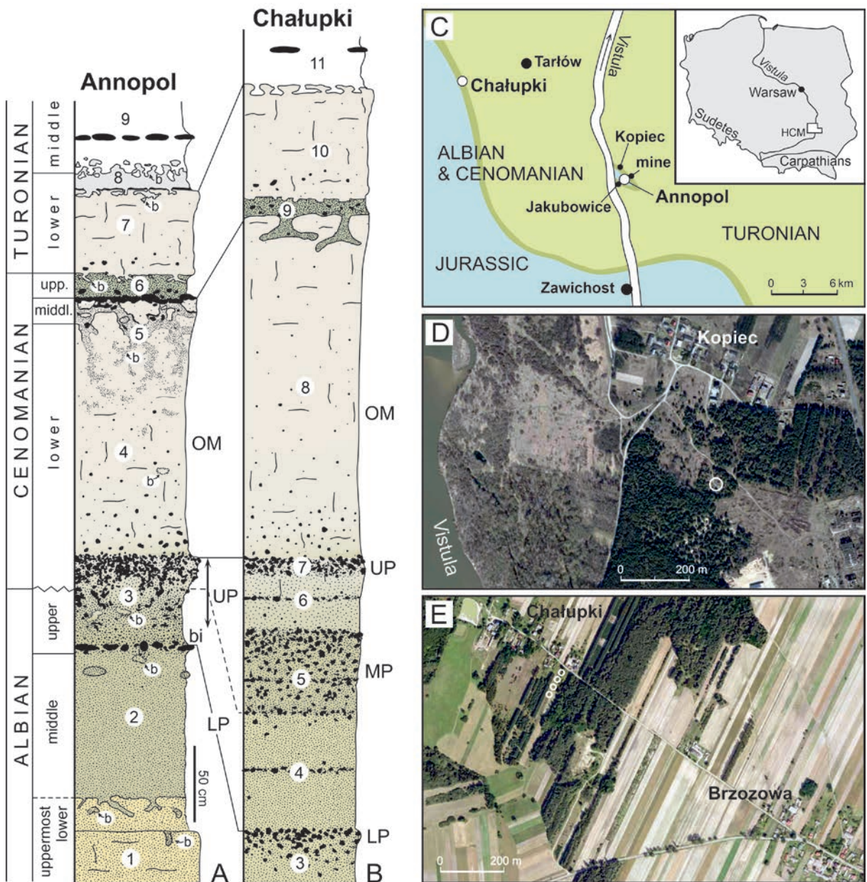
Text-fig. 1. Geological setting and location of the studied outcrops of the phosphorite interval at the northeastern border of the Holy Cross Mts. A – The composite section and subdivision of the Annopol succession based on data from Kopiec and the abandoned underground mine (adapted from Machalski and Kennedy 2013, fig. 1; Kennedy and Machalski 2015, fig. 1 and Machalski and Dubicka 2017, fig. 1, with modifications). B – The composite section of the Chałupki succession (based on this paper). C – Location of the studied area in Poland (insert) and simplified geological map of the study area (adopted from Cieśliński 1959, fig. 1) with marked positions of the localities mentioned in text. D – Location of the Kopiec site (circle) in the Annopol area. E – Location of the Chałupki site (circles). D and E based on the satellite photos, modified from Google Maps. Abbreviations: b – burrow; LP – Lower Phosphorite; bi – ‘baren’ interval; MP – Middle Phosphorite; UP – Upper Phosphorite; OM – Overlying Marls; HCM – Holy Cross Mts. For further explanations see text.
