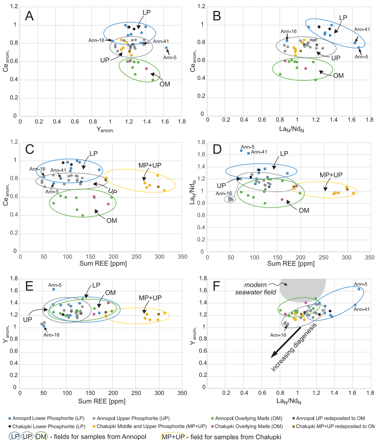
Text-fig. 5. REE composition of studied samples expressed as a combination of parameters. A – Y anomaly vs Ce anomaly. B – La N /Nd N ratio vs Ce anomaly. C – Sum REEs vs Ce anomaly. D – Sum REEs vs La N /Nd N ratio. E – Sum REEs vs Y anomaly. F – La N /Nd N ratio vs Y anomaly.
