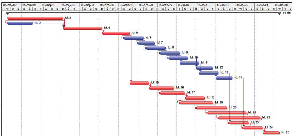
Fig. 2. Schedule of earth works developed for construction of the „A19” metro station with no baseline date being fixed (tasks belonging to the critical path are marked in red)
