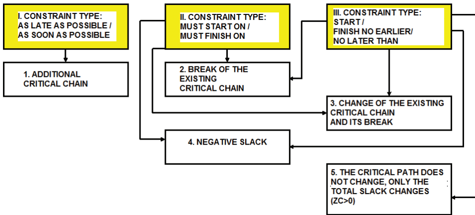
Fig. 1. Diagram of types of constraints with possible consequences of their implementation
