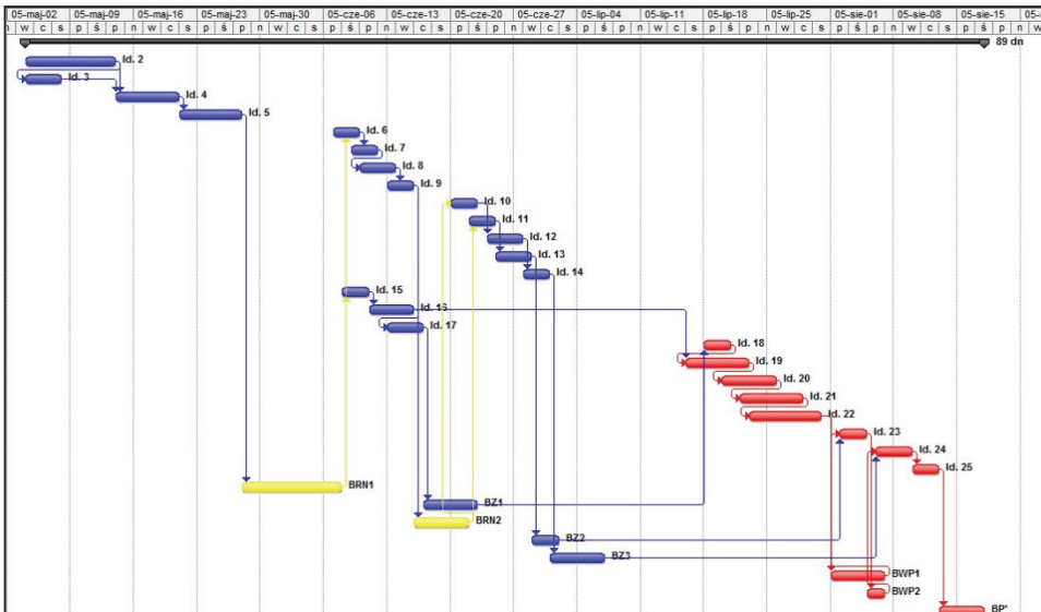
Fig. 6. Gantt chart with the baseline term after insertion of time buffers (shown with their sizes) (tasks lying on the critical path are marked in red).
