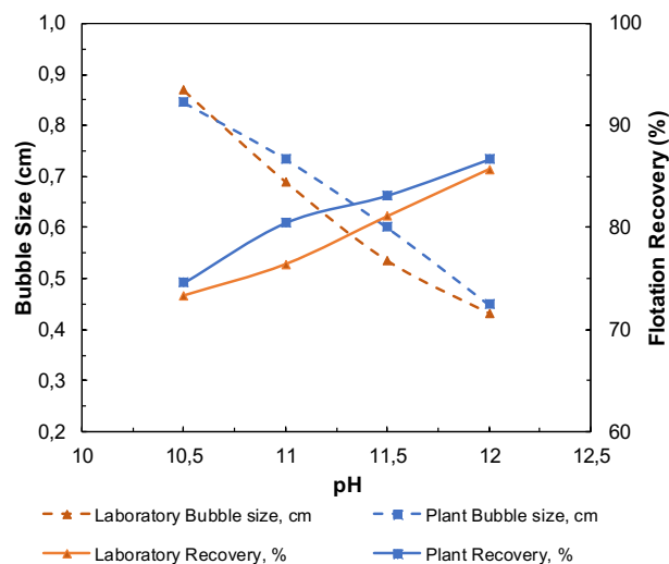
Fig. 13. Effect of pH on bubble size and flotation recovery for laboratory and plant scale experiments
