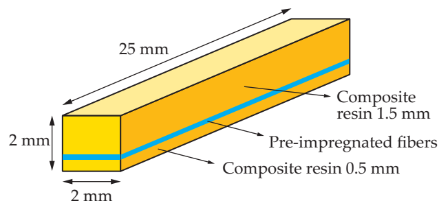
Fig. 1. Shape and measurement of specimens with laminar composite structure
