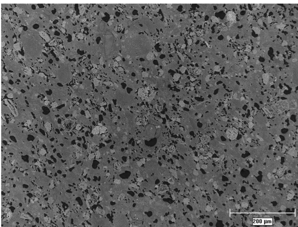
Fig. 3. The structure of C 110 type material of the rod of line post medium voltage insulator of 1981, magnification 100 times. Almost a half of the quartz phase was crashed out, while the mullite phase was not damaged. Intensive cracking inside and around the bright quartz grains is seen
