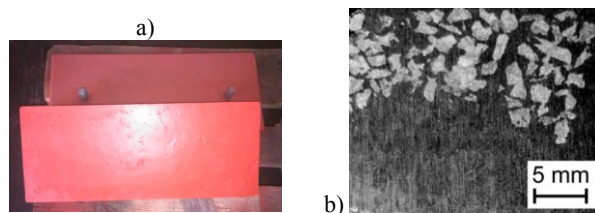
Fig. 8. Castings containing 0,79 kg of electrocorundum grains, two holding-down bolt (a); Composite layer of the thickness of 8 – 12 mm (b)
