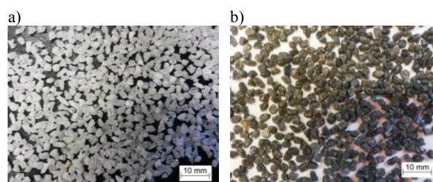
Fig. 1. Ceramic grains: a) white electrocorundum of F12 granularity, b) brown electrocorundum of F10 granularity
