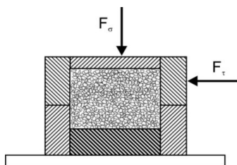
Fig. 4. Plan of test-bed for determination of shear stability in the granular layer [19]
