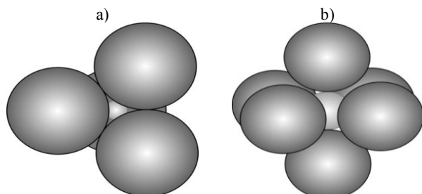
Fig. 2. Types of gaps (pores): a) tetraedric, b) octaedric [22]
