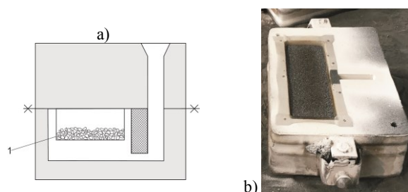
Fig. 6. Cross-section of mould(a) with a layer of stabilized grains (1) on metal mesh; (b) mould drag
