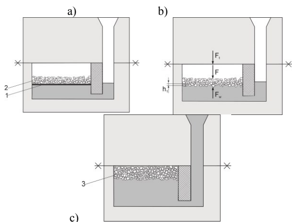
Fig. 5. The possible phases of composite layer production within a hypothetical plate: a) phase I - on the metal mesh (1) the grains lay still (2), their porosity p = 50\% and thickness h = (5; 6) mm, pouring over starts and lasts until the molten metal touches the metal mesh; b) phase II - a temporary resistance of metal flow occurs related to melting of the mesh and penetration into the grain layer to the depth h_1 ; at this moment the buoyancy ( F_w ) balances the gravity of the grains ( F ) and transverse force ( F_t ); c) phase III - elevation of the molten metal in the mold with the layer of grains being created along until it meets the upper limit of the mold, after which, as a result of growing pressure resulting from the height of the upper box the penetration of metal between the grains should occur, thus creating a composite layer
