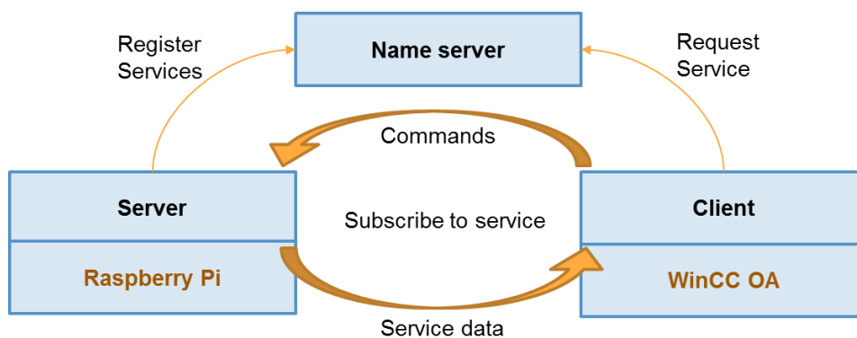
Fig. 1. Communication and data flow between Raspberry Pi and WinCC OA scheme
