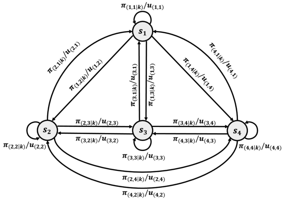
Fig. 1. Pricing Markov chain.
