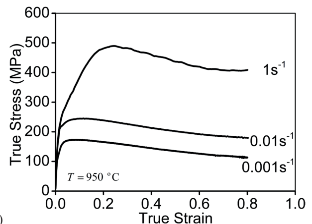
Fig. 2. Typical true stress-true strain curves of the studied superalloy at: (a) \dot{\epsilon}=1\text{s}^{-1} ; (b) T=950^\circ\text{C}
