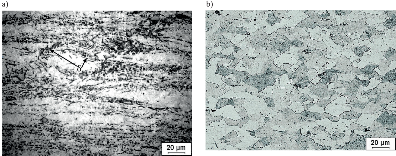
Fig. 12. The high magnification optical microstructure at the strain rate of 0.001s^{-1} and deformation temperatures of: (a) 920^{\circ}C ; (b) 1010^{\circ}C
