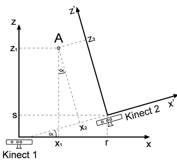
Fig. 3. Relative Kinect transformations for measurement enhancement.
