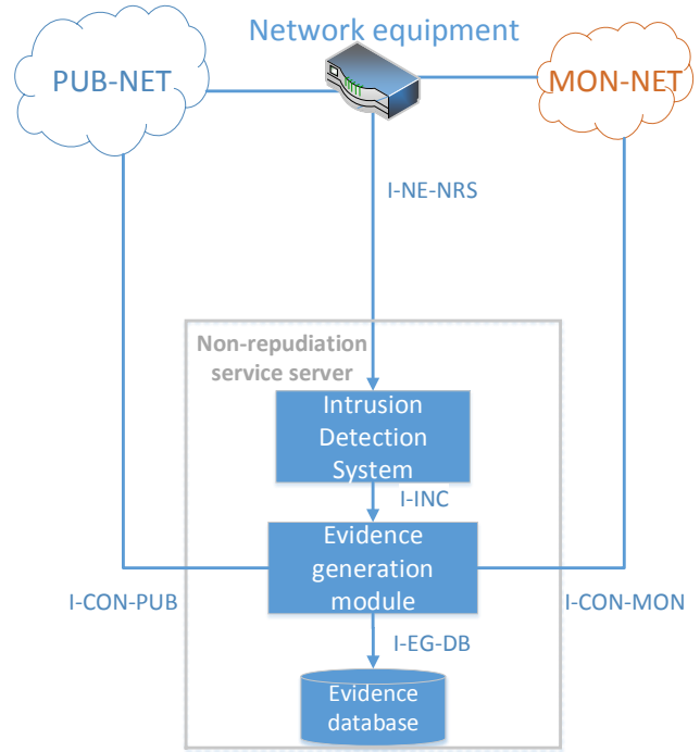
Fig. 5. Implementation architecture
